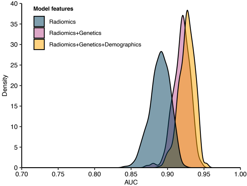
Supplementary Figure 1: Distribution of AUC for classification of IDH mutation status from repeated 5-fold cross-validation using radiomics features unadjusted for potential confounding factors. AUC estimates from 500 random iterations of 5-fold cross validation were obtained from IDH classification models using different combinations of features.
