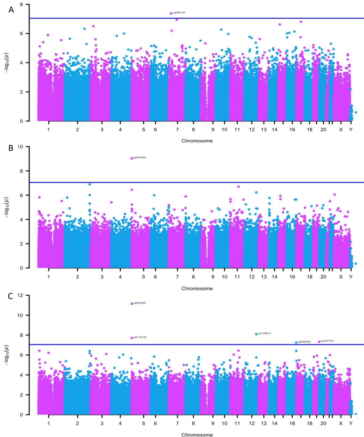
eFigure 2. Manhattan plots of the stratified analyses. Stratified analysis for A) females, B) males, C) European ancestry, D) African ancestry, E) civilian trauma, and F) military trauma. The x-axis depicts chromosomes and the location of each CpG site across the genome. The y-axis depicts the -\log_{10} of the unadjusted p-value for the association with current PTSD. Each dot represents a CpG site. The solid blue line indicates the epigenome-wide statistical significance at p < 9e-8 .
