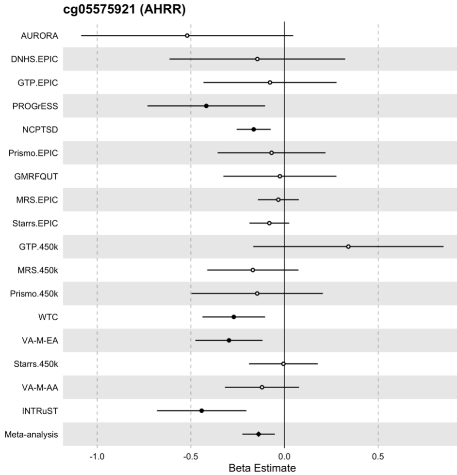
eFigure 4. Forest Plots of CpGs associated with PTSD in the stratified analysis for males. The x-axis is the effect size for each association and includes the 95% confidence interval. Error bars represent the 95% confidence interval, and the center of the error bars represent effect sizes for the CpGs in each cohort. Filled circles indicates a nominally significant association ( p < 0.05 ). Hollow circles indicate the lack of association ( p > 0.05 ). The vertical line indicates an effect size of 0.
