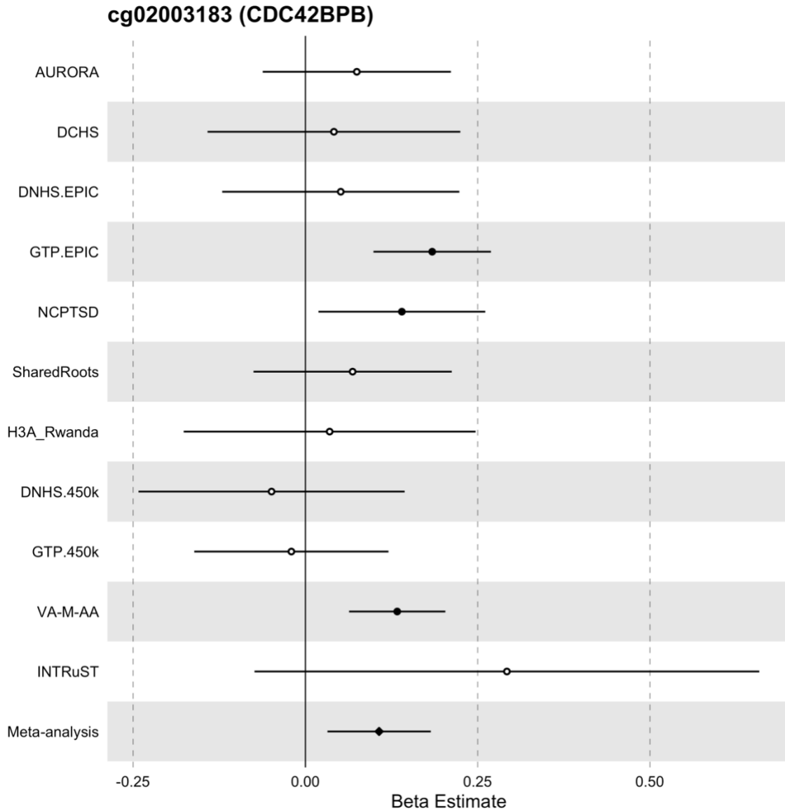
eFigure 6. Forest Plots of CpGs associated with PTSD in the stratified analysis for African ancestry. The x-axis is the effect size for each association and includes the 95% confidence interval. Error bars represent the 95% confidence interval, and the center of the error bars represent effect sizes for the CpGs in each cohort. Filled circles indicates a nominally significant association ( p < 0.05 ). Hollow circles indicate the lack of association ( p > 0.05 ). The vertical line indicates an effect size of 0.
