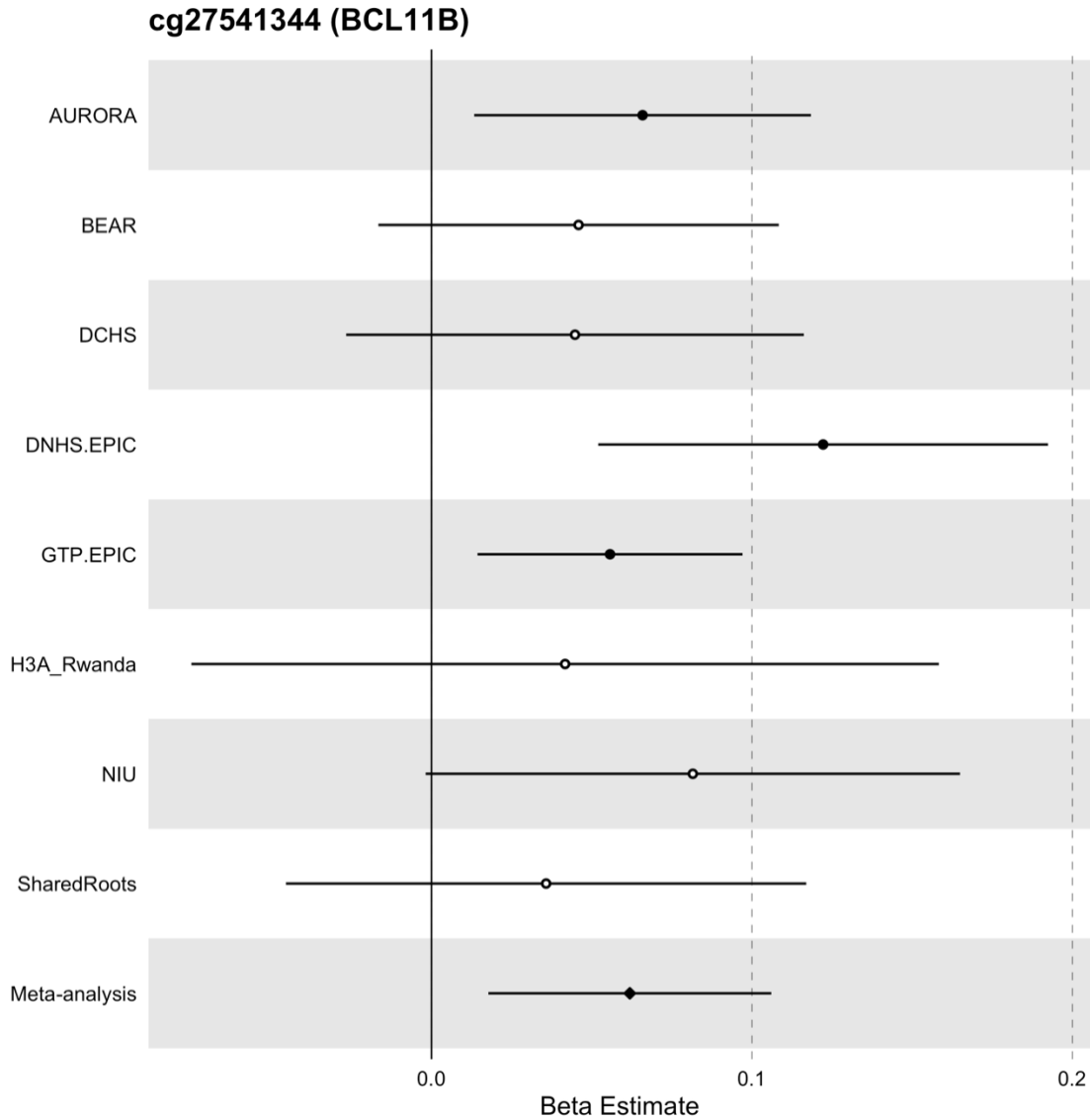
eFigure 7. Forest Plots of CpGs associated with PTSD in the stratified analysis for civilian trauma. The x-axis is the effect size for each association and includes the 95% confidence interval. Error bars represent the 95% confidence interval, and the center of the error bars represent effect sizes for the CpGs in each cohort. Filled circles indicates a nominally significant association ( p < 0.05 ). Hollow circles indicate the lack of association ( p > 0.05 ). The vertical line indicates an effect size of 0.
