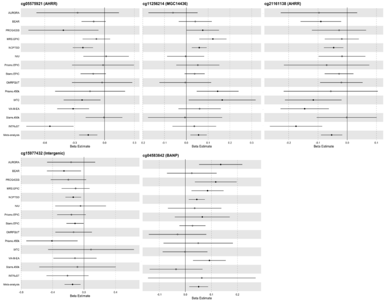
eFigure 5. Forest Plots of CpGs associated with PTSD in the stratified analysis for European ancestry. The x-axis is the effect size for each association and includes the 95% confidence interval. Error bars represent the 95% confidence interval, and the center of the error bars represent effect sizes for the CpGs in each cohort. Filled circles indicates a nominally significant association ( p < 0.05 ). Hollow circles indicate the lack of association ( p > 0.05 ). The vertical line indicates an effect size of 0.
