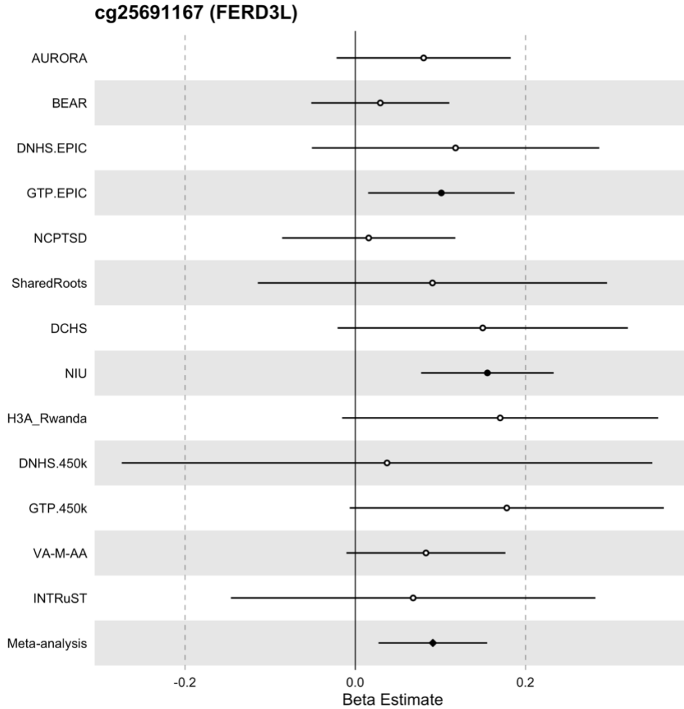
eFigure 3. Forest Plots of CpGs associated with PTSD in the stratified analysis for females. The x-axis is the effect size for each association and includes the 95% confidence interval. Error bars represent the 95% confidence interval, and the center of the error bars represent effect sizes for the CpGs in each cohort. Filled circles indicates a nominally significant association ( p < 0.05 ). Hollow circles indicate the lack of association ( p > 0.05 ). The vertical line indicates an effect size of 0.
