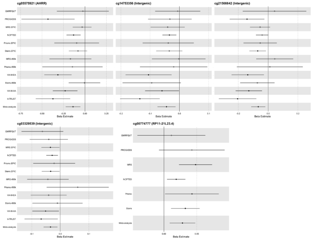
eFigure 8. Forest Plots of CpGs associated with PTSD in the stratified analysis for military trauma. The x-axis is the effect size for each association and includes the 95% confidence interval. Error bars represent the 95% confidence interval, and the center of the error bars represent effect sizes for the CpGs in each cohort. Filled circles indicates a nominally significant association ( p < 0.05 ). Hollow circles indicate the lack of association ( p > 0.05 ). The vertical line indicates an effect size of 0.
