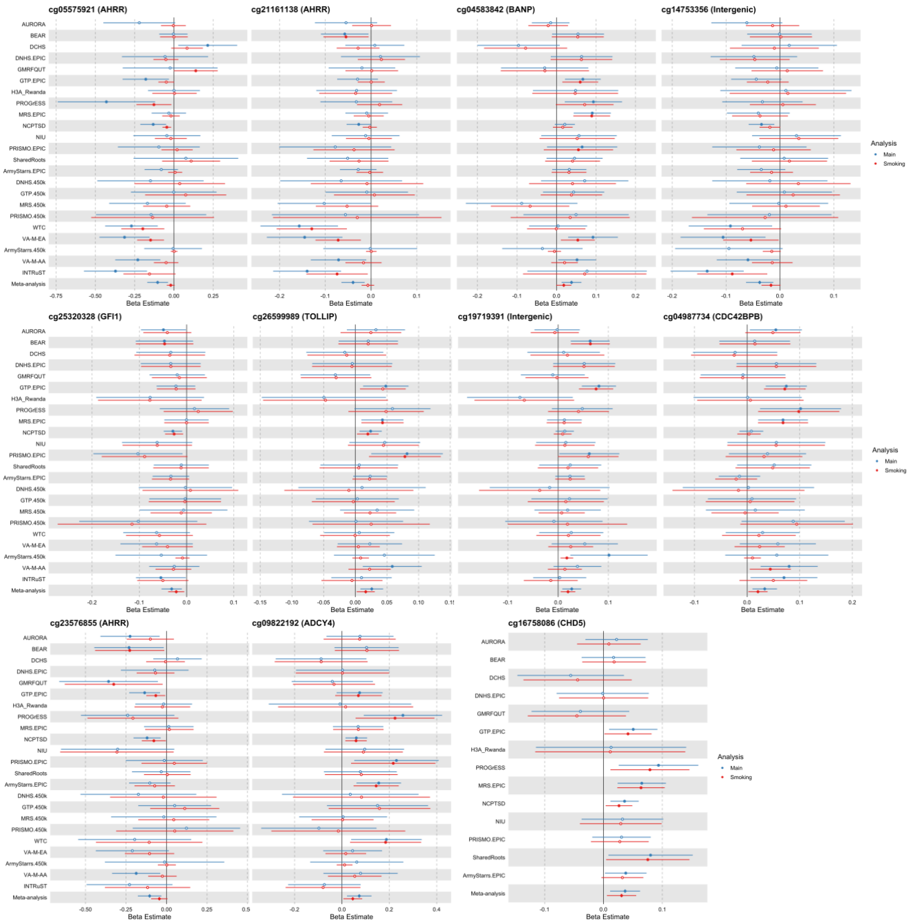
eFigure 1. Forest Plots of PTSD-associated CpGs in each cohort. The x-axis is the effect size for each association and includes the 95% confidence interval. Error bars represent the 95% confidence interval, and the center of the error bars represent effect sizes for the CpGs in each cohort. Filled circles indicates a nominally significant association ( p < 0.05 ). Hollow circles indicate the lack of association ( p > 0.05 ). The vertical line indicates an effect size of 0. Primary meta-analysis is shown in blue and sensitivity analysis for smoking is shown in red.
