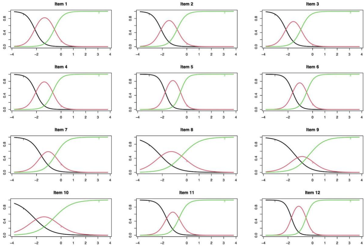
Supplemental Figure S2: Item Response Characteristic Curves (unidimensional solution)
