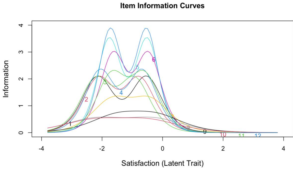
Supplemental Figure S3. Item Information Curves (unidimensional solution)
