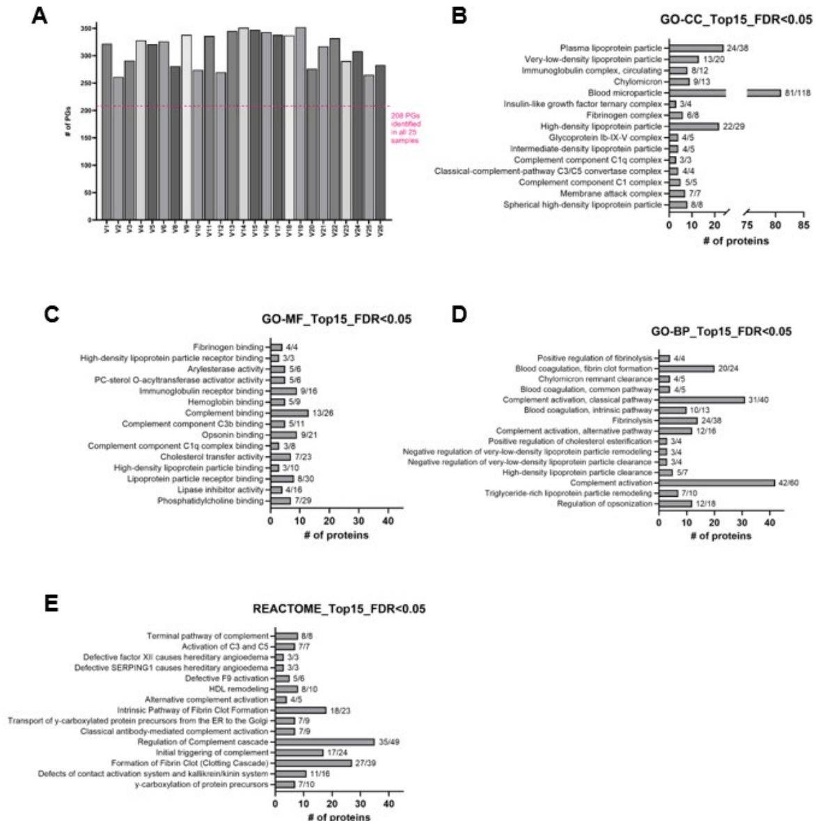
Supplementary Figure 1: Details of protein groups quantified per sample and top scoring pathways and GO annotation
