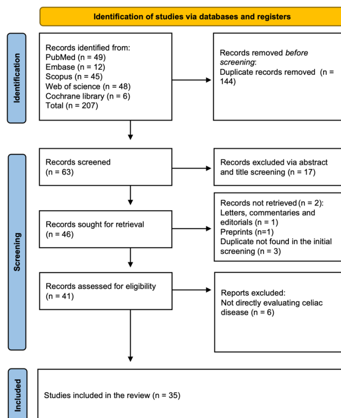
Figure 1: PRISMA flowchart.
