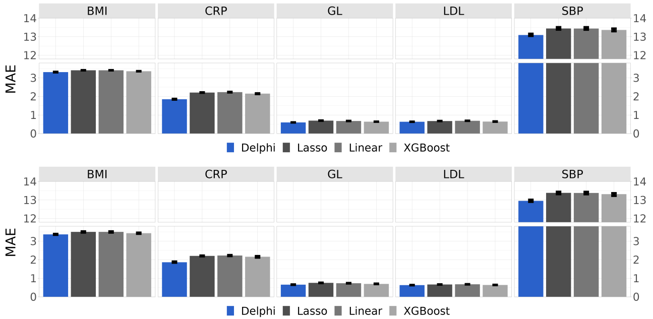
Figure 1. Mean absolute error of polygenic predictions for five phenotypes in the UK Biobank. Top: All participants; bottom: Individuals from non-British white ancestry. We report results for a linear PRS model, lasso regression, an XGBoost model including the dosage of multiple high-impact SNPs as input, and our method. See Figure 2 for acronyms.
