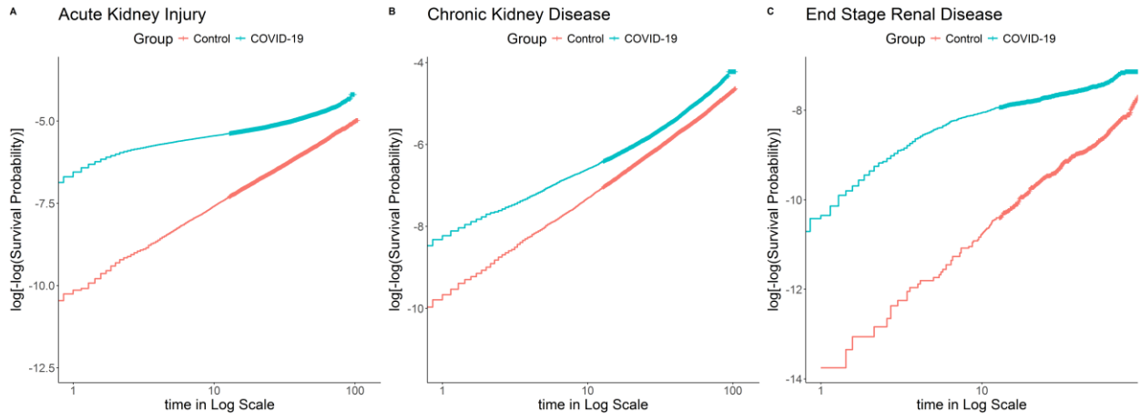
Supplementary Figure 1: log-log survival curves for checking the PH assumption for COVID-19 group and Negative Control groups were almost parallel and the proportional hazard assumption was satisfied
