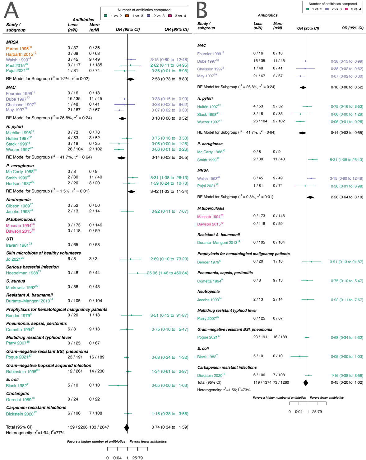
Fig. S1. Forest plot of de novo emergence of bacterial resistance stratified by the reason antibiotics were administered. The coloring indicates the number of antibiotics that were compared in each study. A) The overall pooled LOR of all included studies. B) The pooled LOR of studies with at least one antibiotic in common in the treatment arms. MRSA stands for methicillin-resistant Staphylococcus aureus , MAC for Mycobacterium avium complex, and BSI for blood stream infection.
