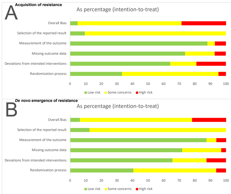
126 Fig. S2. Risk of bias summary for the two main outcomes: A) Acquisition of resistance, B) de 127 nov o emergence of resistance.
