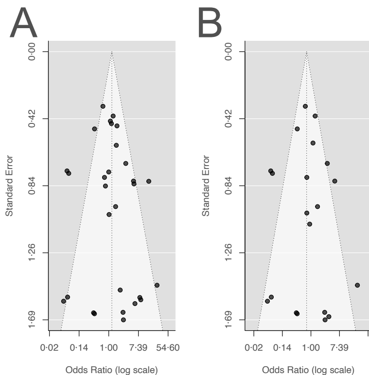
192 Fig. S5. Funnel plots for the two main outcomes: A) acquisition of resistance, B) de novo 193 emergence of resistance.
