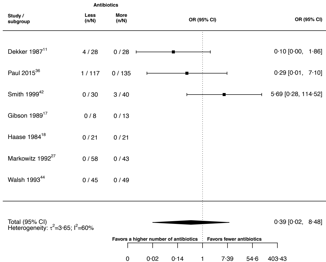
649 650 Fig. S13. Forest plot of acquisition of resistance against non-administered antibiotics. 651
