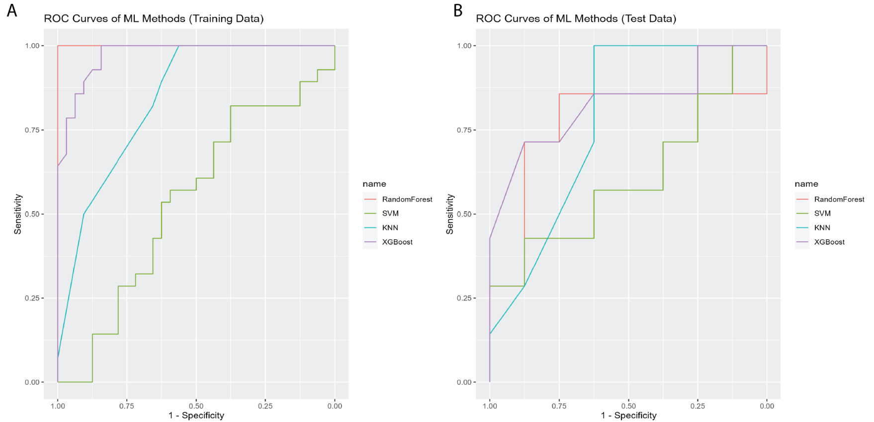
Figure 2. The comparison of prediction performance. (A) Evaluation of machine learning methods' prediction ability using ROC curves to distinguish AFib patients from controls in the training dataset. (B) Evaluation using test datasets.
