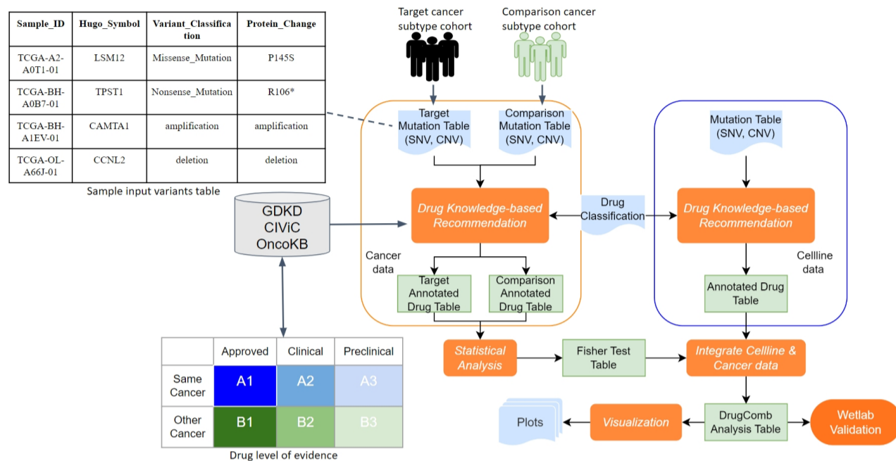
Fig. 2. The workflow for Onko_DrugCombScreen drug combination data analysis. After the recommendation process based on drug knowledge, SNVs and CNVs are merged into an annotated drug table. Following statistical analysis and integration of cell line data, the final DrugComb analysis table will be used for visualization and wet lab validation.
