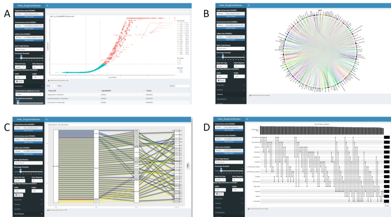
Fig. 3. Visualization of the Onko_DrugCombScreen. (A) Volcano plot identifying significant drug combinations. (B) Circle plot depicting the most proportional drug co-recommendations. (C) Alluvial diagram tracing mutations back to recommended single drugs. (D) UpSet plot showing the top-recommended single drugs and their intersections.
