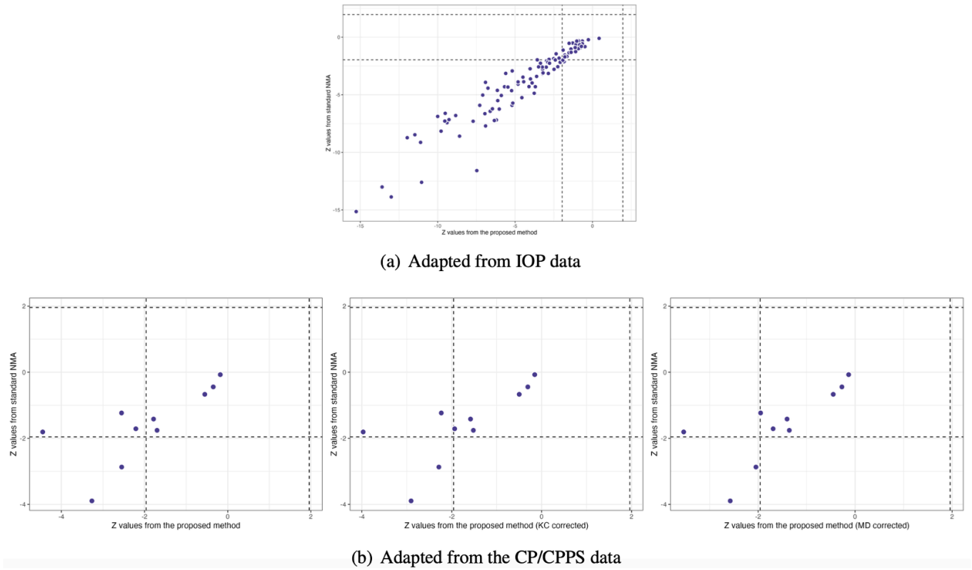
Figure 5: Comparisons of Z values using the standard NMA based on the Lu and Ades' approach, the proposed method without any corrections, and the proposed method with KC-corrected or MD-corrected sandwich variance estimators, respectively
