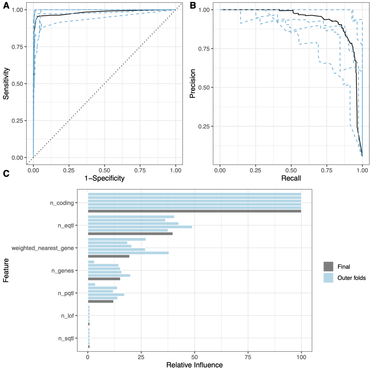
Supplementary Figure 5. Performance of V2G scoring model. A. ROC performance curve. Lighter colored curves show ROC performance per outer CV fold; B. PR performance curve. Lighter colored curves show PR performance per outer CV fold; C. Relative importance for each feature used in the model, as described in Friedman (2001) 2 and implemented in the gbm package in R.
