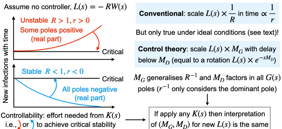
Fig 1: Epidemic architecture and controllability definition. Panel A shows that the renewal epidemic model is a positive feedback system with signals being successively fed back along
