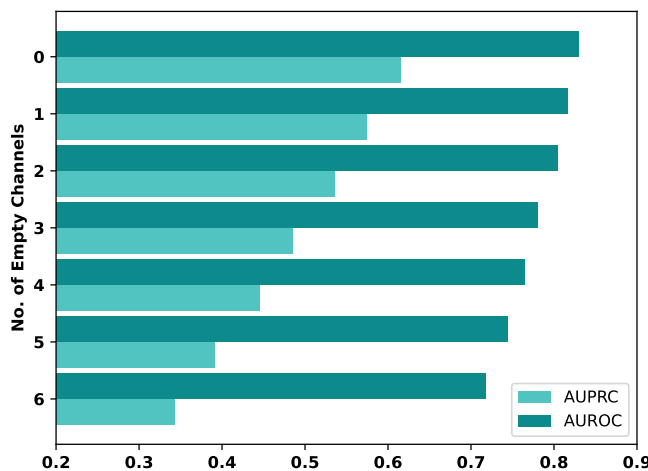
Figure 4: Assessing model robustness using AUROC and AUPRC metrics across different levels of missing channels in CPSC ECG data.
