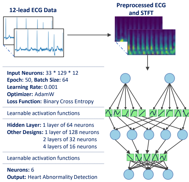
Figure 2: The model architecture consists of KAN neurons tailored for STFT-processed ECG data. The input layer comprises 33 \times 129 \times 12 neurons, matching the STFT pre-processed ECG data points. It then passes through intermediate layers with 64 neurons, with additional intermediate architectures also tested. Finally, six output neurons are corresponding to the six abnormalities being detected.
