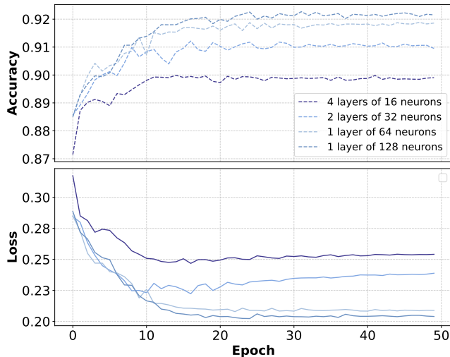
Figure 3: The training processes of various KAN architectures show increasing accuracy and decreasing loss throughout. However, discrepancies can be observed among different network architectures.
