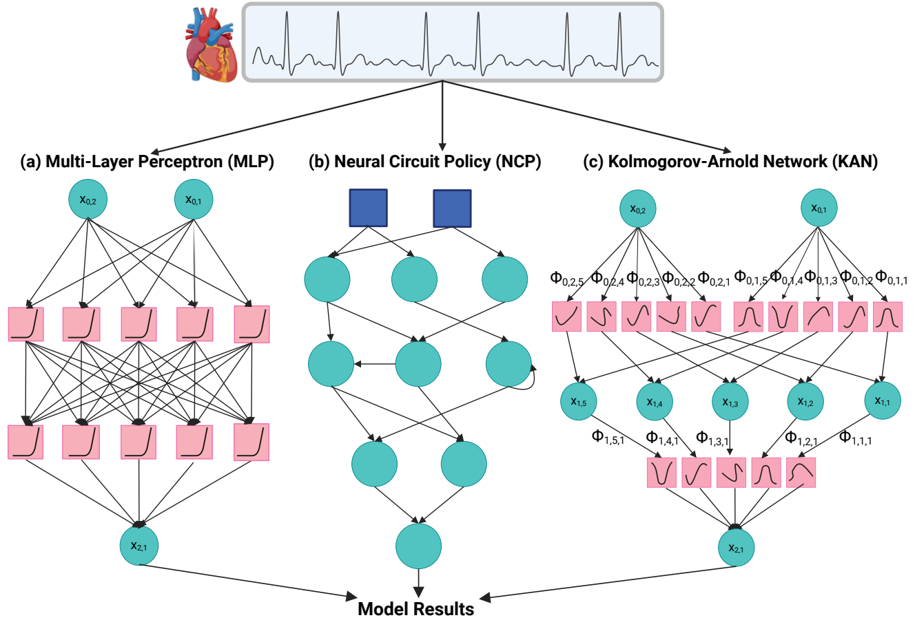
Figure 1: The figure illustrates the distinctions between three types of networks: a traditional Multilayer Perceptron (MLP) with a pre-set activation function (a), a Neural Circuit Policy (NCP) designed to emulate biological neural circuits (b), and a KAN network capable of learning activation functions (c). (a) Represents a standard MLP architecture where the activation functions are predetermined and fixed. (b) Depicts an NCP model that mimics biological neural circuits’ modularity and information flow, emphasizing adaptability and task-specific decision-making. (c) Shows a KAN network with the unique ability to learn and adjust its activation functions based on the input data and learning objectives, enhancing its flexibility and performance across diverse tasks.
