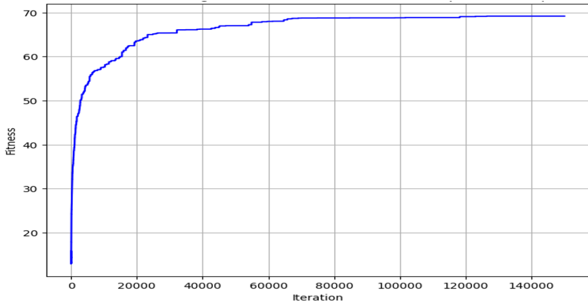
Supplement 4: Optimization curve of DGESA applied on UC vs. Normal dataset: 40 Discriminative Genes in UC were found using an optimization process. The optimization procedure to identify a subset of 40 genes that together optimize the discrimination between the UC and control samples in the gene expression dataset is depicted in this image. The graph illustrates how the optimization process is convergent and stabilizes at about 70,000 epochs.
