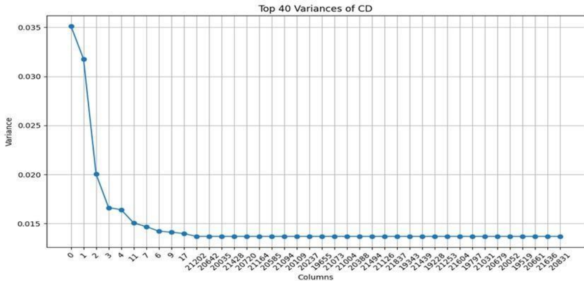
Supplement 1: Variance of Top 40 Genes in CD vs. normal Gene Expression Data: The variance of the top 40 genes in the CD gene expression dataset is displayed as a line plot in this figure. The genes with the highest variation are represented by their indices on the x-axis, and their variance values are displayed on the y-axis. The graphic shows that the variance of the first few genes is very high and then flattens off for the next genes.
