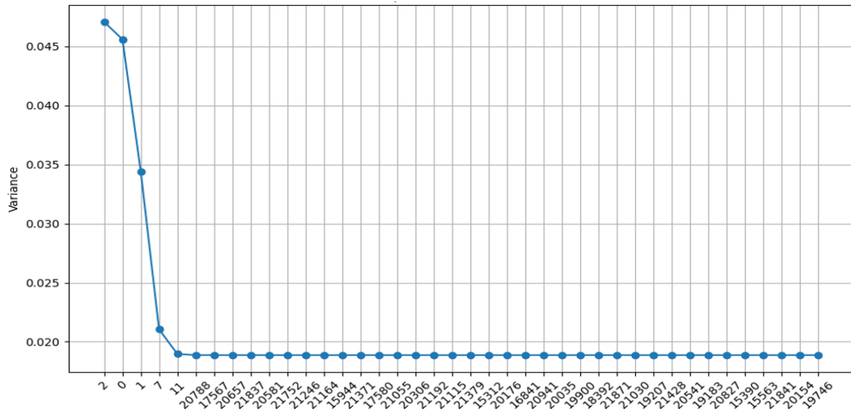
Supplement 2: Variance of Top 40 Genes in UC Gene Expression Data: The gene expression dataset's variance for the top 40 genes is plotted as a line graph in this picture. The y-axis shows the variance values, while the x-axis shows the indices of the genes with the highest volatility. Plotting shows that a very high variation is seen in the first few genes and then flattens out for the next genes.
