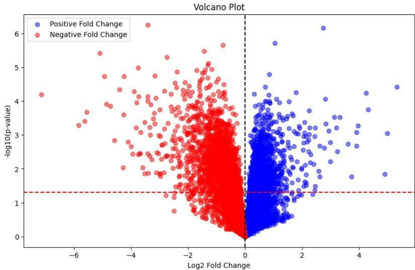
Figure 3. Volcano Plot of Gene Expression Data for EOE: This figure presents a volcano plot illustrating the gene expression data for EOE. The x-axis represents the log 2 fold change, while the y-axis denotes the -log 10 P-value. The plot highlights a greater number of genes with negative fold changes compared to those with positive fold changes, indicating differential gene expression patterns in EOE.
