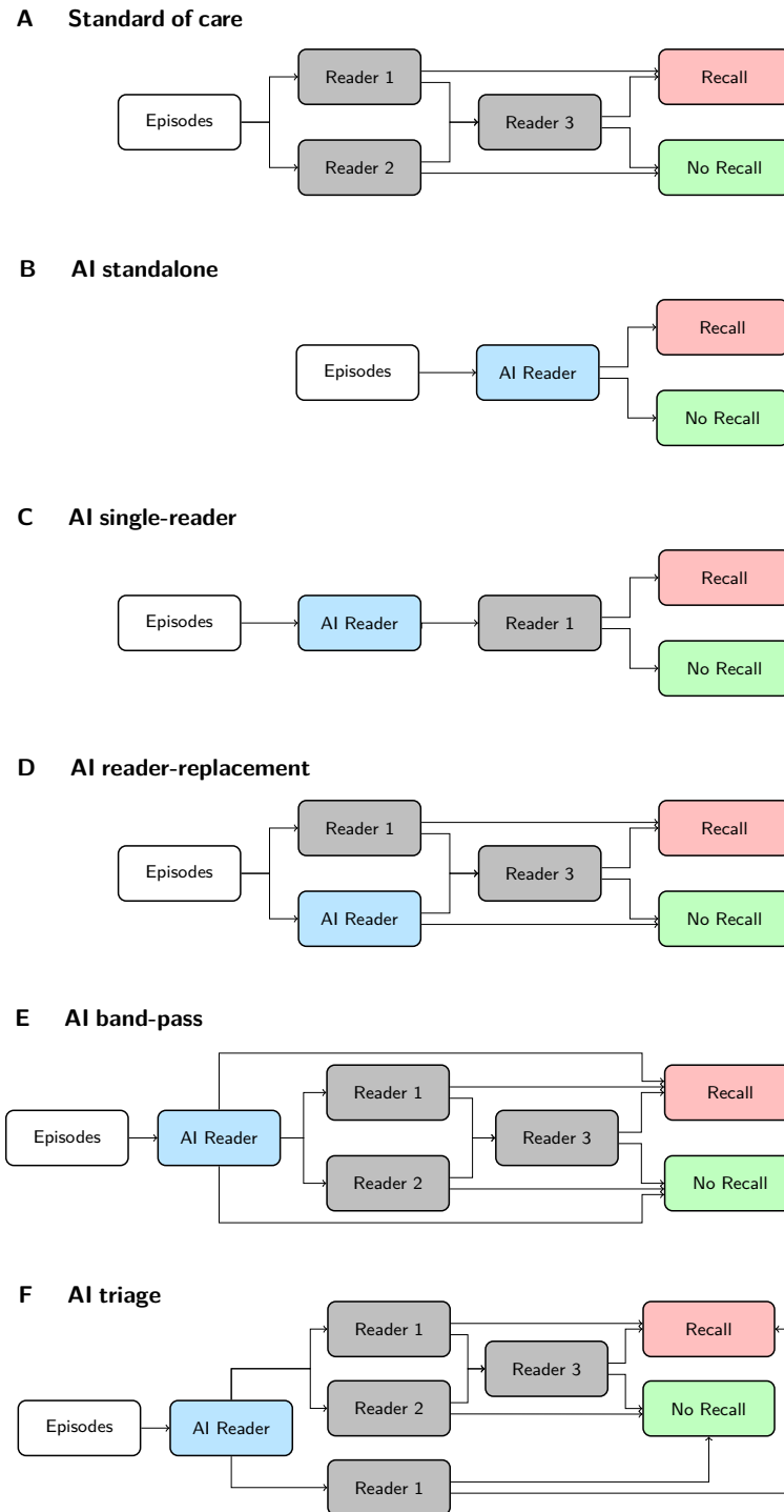
Figure 1. Screening episode flows for the current reader system and AI integration scenarios. (A) Standard of care scenario: Readers 1 and 2 see the same episode and opt to recall or not-recall, if they disagree Reader 3 arbitrates. (B) AI standalone scenario: all decisions are taken by the AI Reader without human intervention. (C) AI single-reader scenario: Reader 1 takes the final decision using AI Reader input. (D) AI reader-replacement: same as (A) but with AI Reader replacing Reader 2. (E) AI band-pass scenario: AI Reader screens out episodes before Readers 1 and 2. Episodes with high scores trigger the recall decision directly, and episodes with low scores trigger the no-recall decision directly. The other episodes continue to the usual reader system. (F) AI triage scenario: AI reader triages the episodes before Readers 1 and 2. Episodes with high scores continue to the usual system, and episodes with low scores go through the path with only 1 reader.
