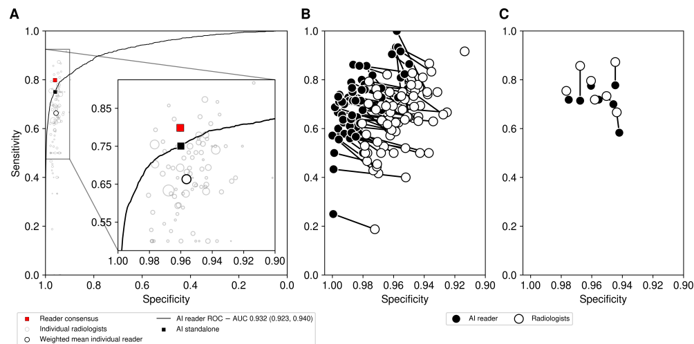
Figure 2. Performance of the AI reader on retrospective cohort. (A) The AI reader ROC curve compared with the weighted mean individual reader and reader consensus for 149,105 screening episodes. The AI reader achieved an AUC of 0.932 (95% CI 0.923, 0.940) above the weighted mean individual reader performance (95.6% specificity, 66.7% sensitivity) but below the reader consensus performance (96.1% specificity, 79.8% sensitivity; standard of care). The weighted mean individual reader (black circle) is the mean sensitivity and specificity of all the individual readers (grey circles; 125 readers) weighted by their respective total number of reads. (B) and (C) AI reader compared against 81 individual readers (min. 1,000 reads). An optimal point from each AI reader ROC curve is shown for each comparison. We show separately human readers for which both sensitivity and specificity of the AI reader point was greater than or equal to the reader (B; 74 readers, 91.3% of readers; 253,328 reads, 88.3% of reads) and readers for which the AI reader is less than or equal to the human reader in either sensitivity or specificity (C; 7 readers, 8.6%; 33,525 reads, 11.7%).
