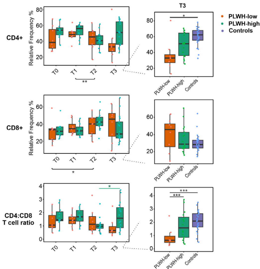
Figure 3. Evolution of CD4+, CD8+, and CD4:CD8 T-cells in PLWH and controls vaccinated with BNT162b2 vaccine. PLWH were studied from T0 till T3, while the controls were only studied at the last time point. Overall frequencies of CD4+ T cells of PLWH-high and PLWH-low were not significantly different during the study period, suggesting stable HIV disease status. Green statistical line represents the significance of pairwise comparisons overtime within PLWH-high group. Black significance lines under the plot represents significant groupwise comparisons overtime of PLWH group. Box plots indicate median (middle line), 25th and 75th percentile (box), and the 5th and 95th percentile (whiskers). All data points, including outliers, are displayed. PLWH, people living with HIV; T0: prior to the 1st dose vaccine; T1: prior to the 2nd dose; T2: 3 months after 2nd dose; T3: 6 months after 2nd dose. *: p < 0.05. **: p < 0.01. ***: p < 0.001.
