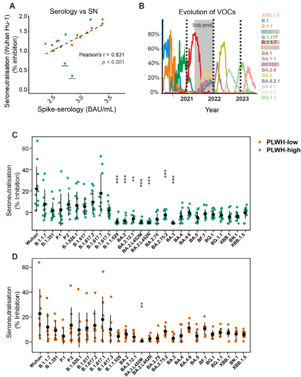
Figure 2. Anti-SARS-CoV-2 serological and seroneutralization responses in PLWH vaccinated with BNT162b2 vaccine. (A) Correlation between anti-RBD Serology and neutralization of Wuhan variant at 3 months after the second vaccination (T2). Two PLWH-low participants had high anti-RBD titers but neutralization potential was poor, marked with a black line. (B) Circulating VOCs in Italy during the study period. (C and D) Anti-Spike neutralization in PLWH-high and PLWH-low against different VOCs measured at T2. Dot plots indicate mean and whiskers indicate 1 standard deviation. **: p < 0.01 . ***: p < 0.001 .
