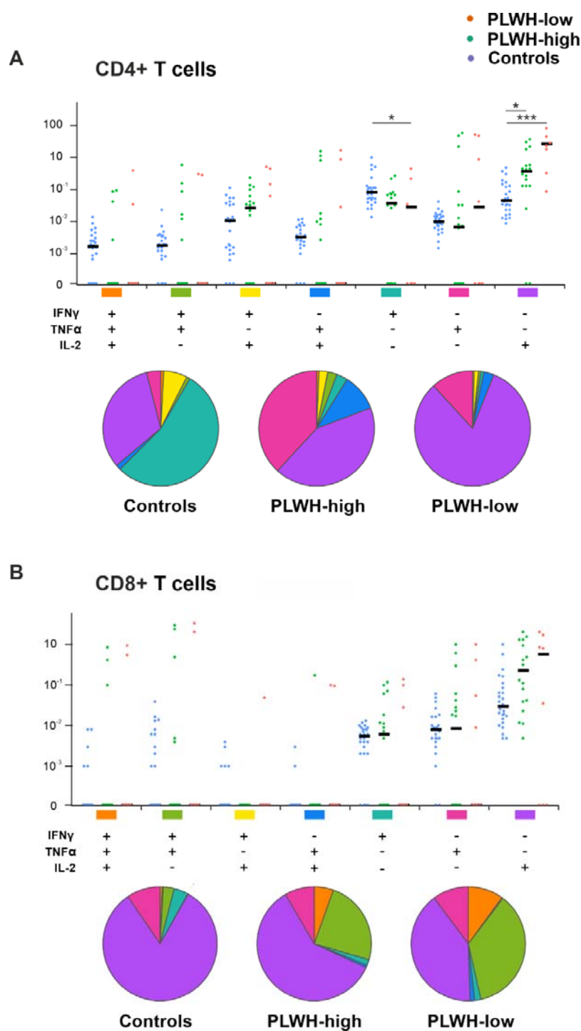
Figure 4. Impact of BNT162b2 vaccination on SARS-CoV-2 spike specific polyfunctional cytokine expression profiles in CD4 + and CD8 + T-cells. Profiles of individual and simultaneous cytokine expression in PLWH and HIV-negative control participants vaccinated with BNT162b2 vaccines analysed at 6 months after the second vaccination (T3) after stimulating with SARS-CoV-2-specific S- peptides. The size of each pie segment relates to the frequency of a monofunctional, bifunctional and triple-functional response. Statistics was performed using SPICE software for polyfunctionality assessment (see Methods).
