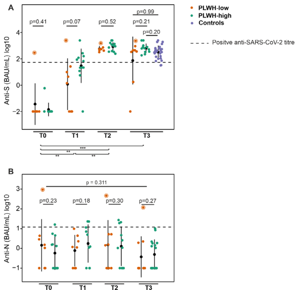
Figure 1. Anti-SARS-CoV-2 serological responses in vaccinated PLWH population stratified as PLWH-high and PLWH-low. (A) Anti-RBD (Wuhan Hu-1) IgG titers measured using the Roche Elecsys anti-SARS-CoV-2 immunoassay in paired serum samples of PLWH-high and PLWH-low following vaccine administration. Roche Elecsys detection limit = 2500 BAU/mL. (B) Anti-Nucleocapsid IgG titers measured using MSD assay in paired samples of PLWH-high and PLWH-low. Control samples were not analysed for anti-N IgG. Dot plots indicate mean (black dot) and 1 standard deviation (whiskers) for (A) and (B). The dashed line indicates the positive SARS-CoV-2 titers for each assay. All data points, including outliers, are displayed. **: p < 0.01 . ***: p < 0.001 . Highest titers for anti-N and anti-S antibodies was noted for one PLWH-low participant who was likely infected before receiving the first dose (circled dot). T0: Pre-vaccination timepoint; T1: 1 month after the first vaccination; T2: 3 months after the second vaccination; T3: 6 months after the second vaccination.
