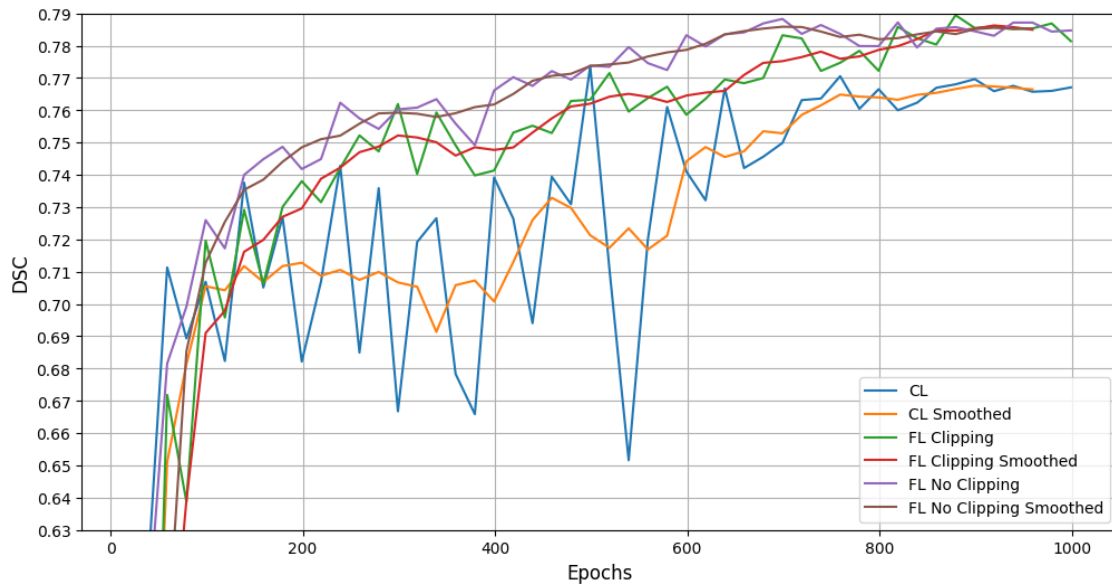
(c) Test DSC
