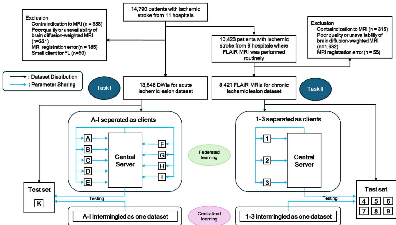
Figure 1. Study flow chart and study scheme for Task I, II. Blue arrows indicate the flow of model parameters, disseminated from the central server, trained by each client, and submitted to the server again. Exact distribution of the data can be found in the supplementary materials.
