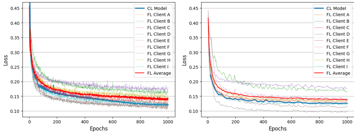
(a) Train Loss
