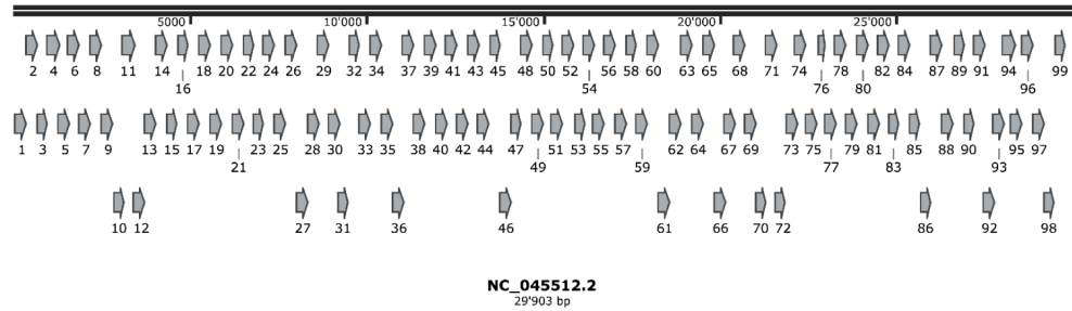
Supplementary Figure A: (a) Positional coverage of the SARS-Cov-2 (NC_045512.2) by sequencing technology. (b) Schematic representation of the distribution of the amplicons resulting from the v4.1 ARTIC primers over the SARS-Cov-2 genome (NC_045512.2).
