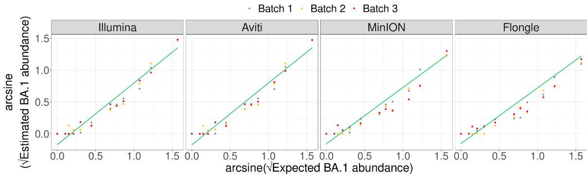
Supplementary Figure I: Comparison of expected and estimated BA.1 abundance for re-normalized data on arcsine-square root scale. The green line represents the derived linear model, for more information see Methods.
