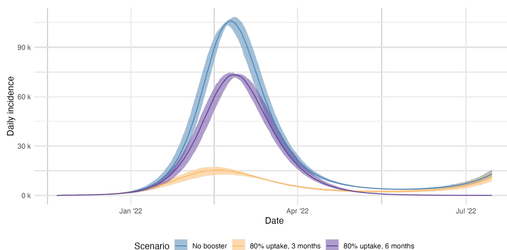
Fig 6. Daily incidence of all infections for the Delta variant only under alternative immunisation scenarios. We compare no boosting as a baseline with 80% of the primed (vaccinated) population for either the (initial) 6 or (proposed) 3 month delay to booster eligibility.
