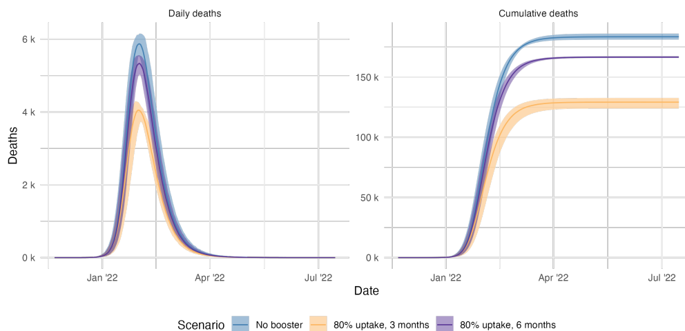
Fig 13. The daily and cumulative deaths for the projected Omicron wave.
