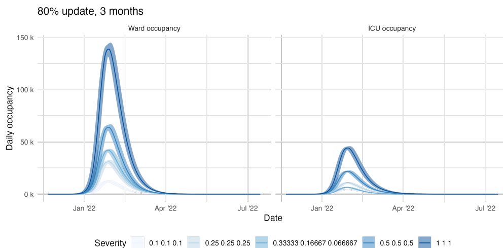
Fig 10. The effect of reduced levels of severity on the clinical outcomes pathways.
