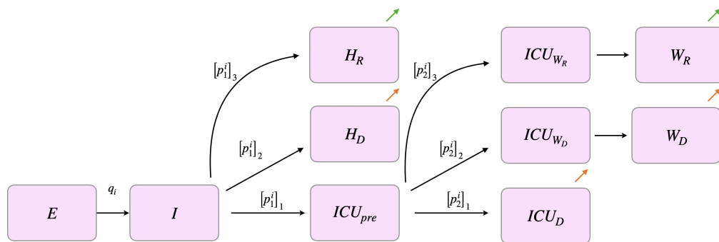
Fig 2. Diagram representing the transitions an individual can make in the clinical pathways model. Transitions resulting in discharge and death are represented with green and orange arrows.
