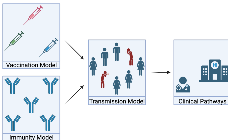
Fig 1. Schematic demonstrating how each component of the model is linked together. First the vaccination allocation is determined and the immunity model is calibrated to real world data. This information is linked into the transmission model, which simulates the spread of COVID-19. Finally, the infections from the epidemic model are linked to the Clinical Pathways model. Created with BioRender.com
