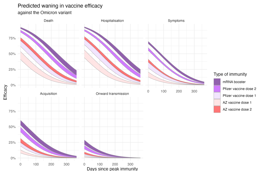
Fig 4. Estimated levels of protection for all outcomes of interest against the Omicron strain (modified from [12]). The bands correspond to the 90% confidence interval.
