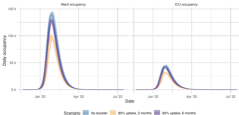
Fig 12. The ward and ICU occupancy levels for the projected Omicron wave, assuming the same severity as the delta strain.
