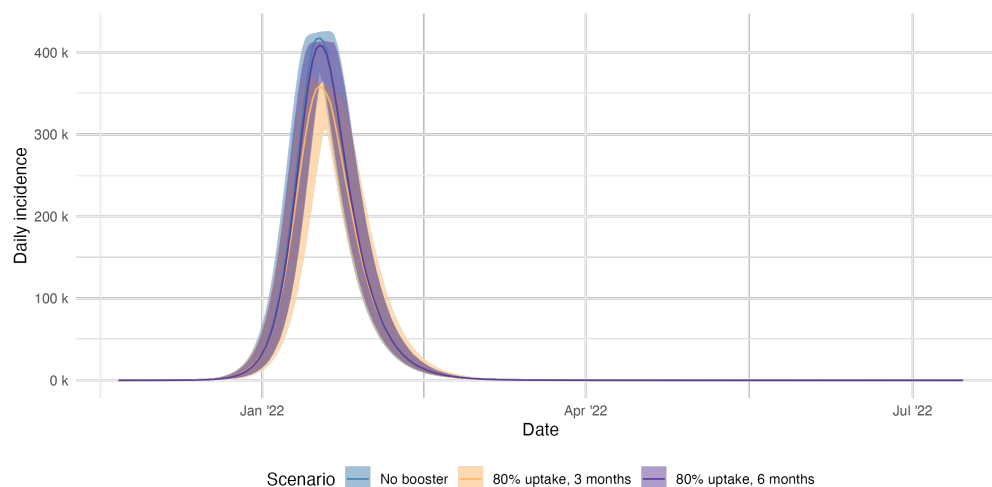
Fig 9. Simulated daily incidence of infections for the Omicron variant only under alternative immunisation scenarios. We compare no boosting as a baseline with 80% of the primed (vaccinated) population for either the 6 or 3 month delay to booster eligibility.
