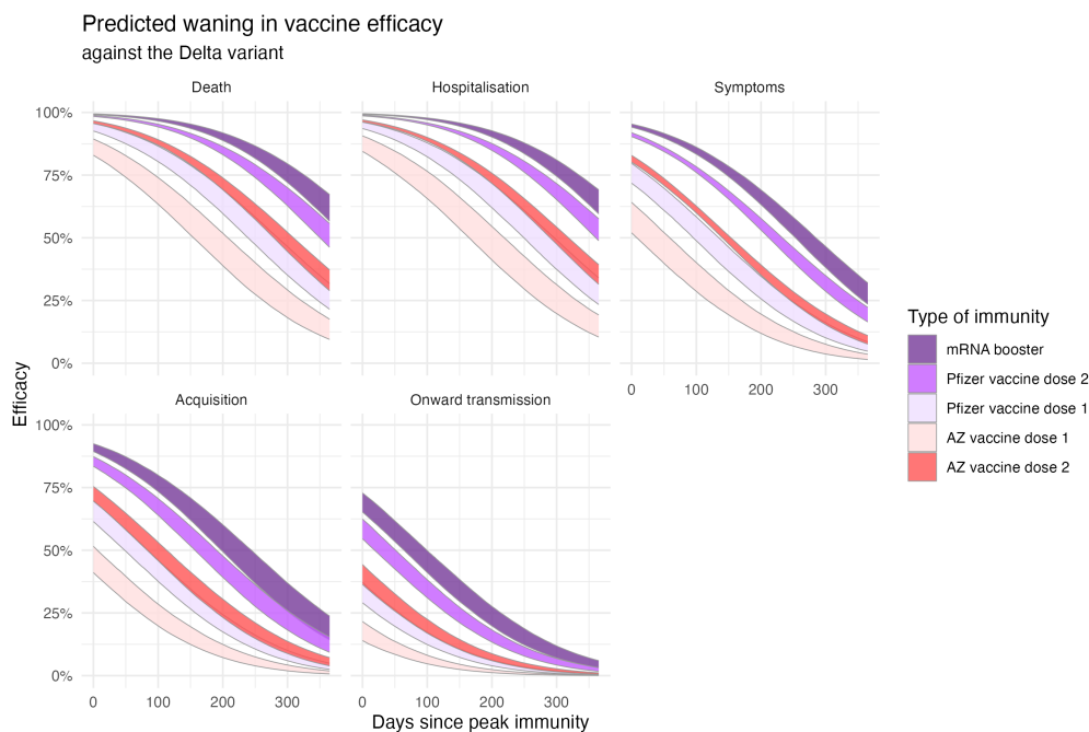
Fig 3. Estimated levels of protection for all outcomes of interest against the Delta strain (modified from [12]). The bands correspond to the 90% confidence interval.
