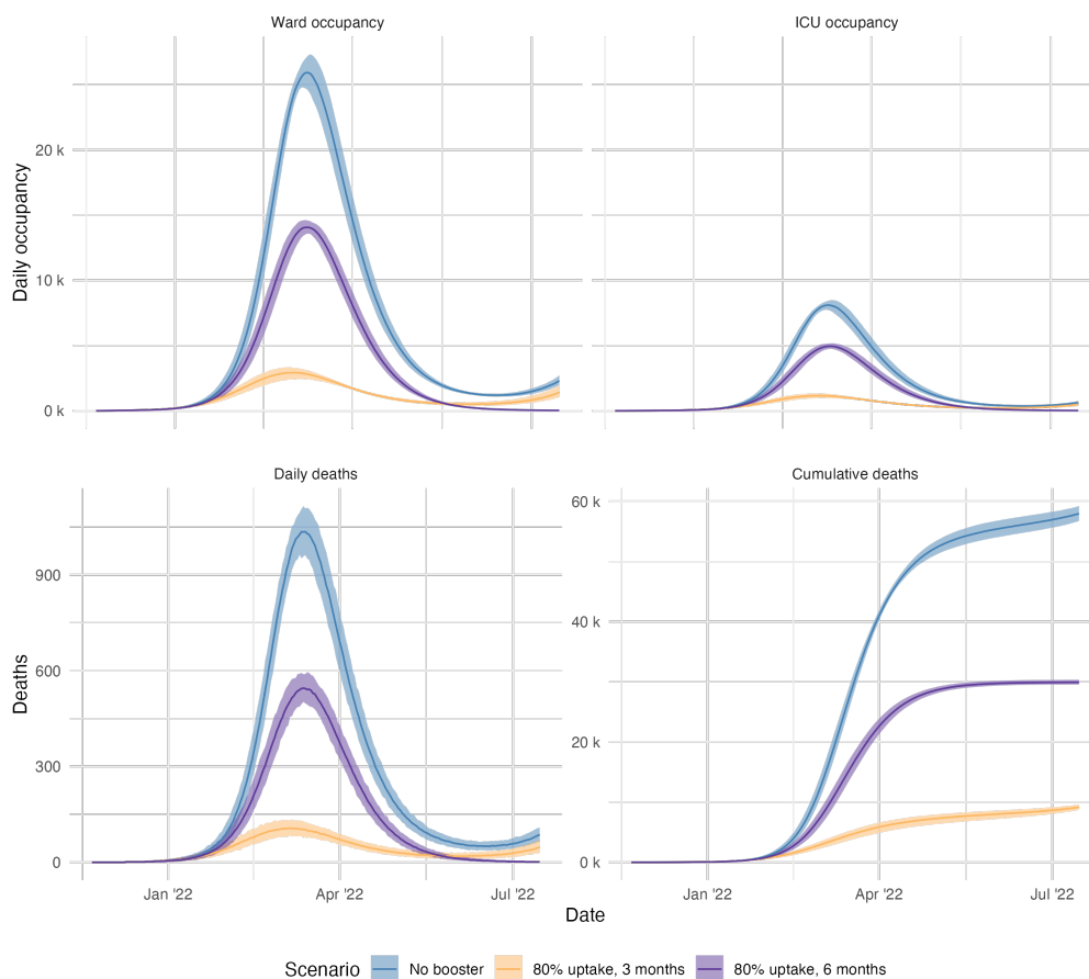
Fig 8. Simulated Ward and ICU occupancy as well as the daily and cumulative deaths for each Delta scenario.
