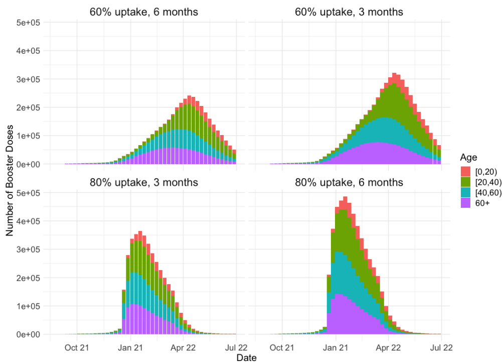
Fig 5. Daily number of booster doses administered in four representative age groups. Due to the age structured administration of the primary course, we can see that younger individuals receive their booster doses after older individuals.
