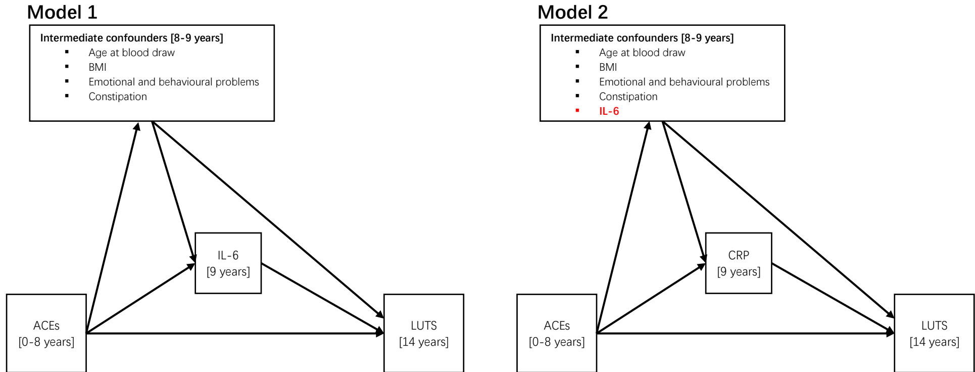
Supplementary Figure 1 Directed acyclic graph (DAG) of mediation model 1 and model 2
