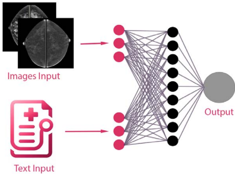
Figure 5. An illustration of a multimodal deep learning model. This diagram demonstrates the integration of a clinical note (textual data) and contrast-enhanced mammography images (visual data) within a neural network architecture. These are processed through distinct pathways before being merged in a unified framework, facilitating a comprehensive analysis in the context of patient diagnosis.
