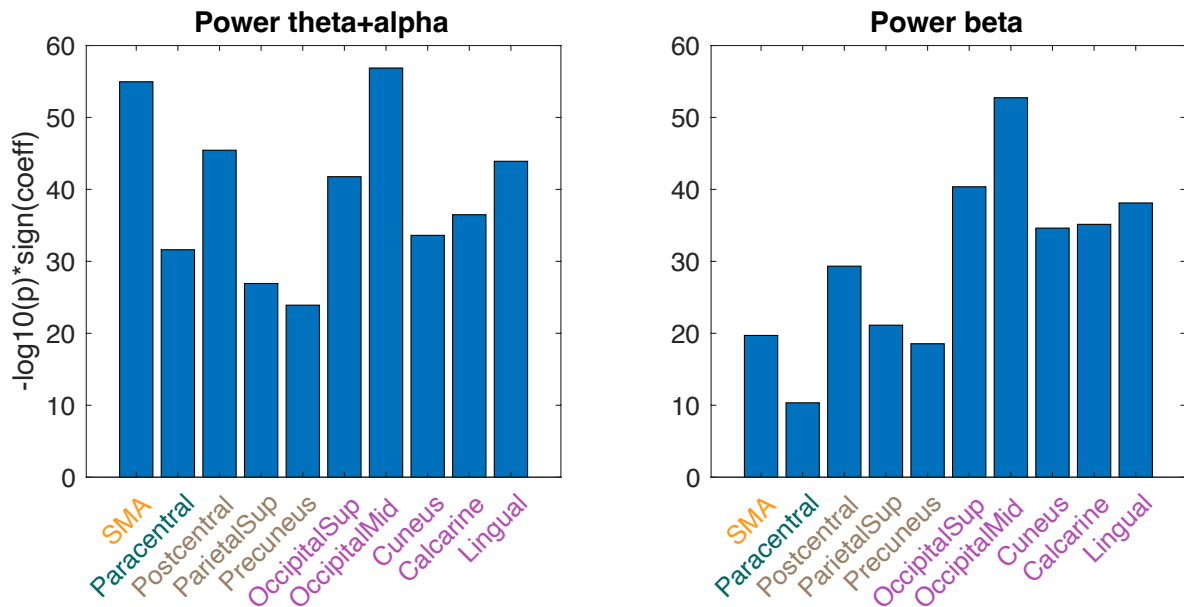
Figure S1. Comparison of EEG power between resting and walking conditions in the theta-alpha and beta bands. We show \log_{10} p -values, thus values below -2 and above 2 would indicate significance at alpha level 0.01. Signed \log_{10} p -values that were not significant after FDR correction are set to zero.
