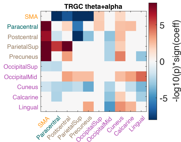
Figure S2. Comparison of EEG markers between resting and walking conditions in the theta-alpha band. Changes in directed functional connectivity were estimated by time-reversed Granger causality (TRGC). Red colors either indicate more information flow from the ROI on the Y-axis to the ROI on the X-axis in walking compared to resting, or less information flow from the ROI shown on the X-axis to the ROI shown on the Y-axis. We show \log_{10} p -values, thus values below -2 and above 2 would indicate significance at alpha level 0.01. Signed \log_{10} p -values that were not significant after FDR correction are set to zero.
