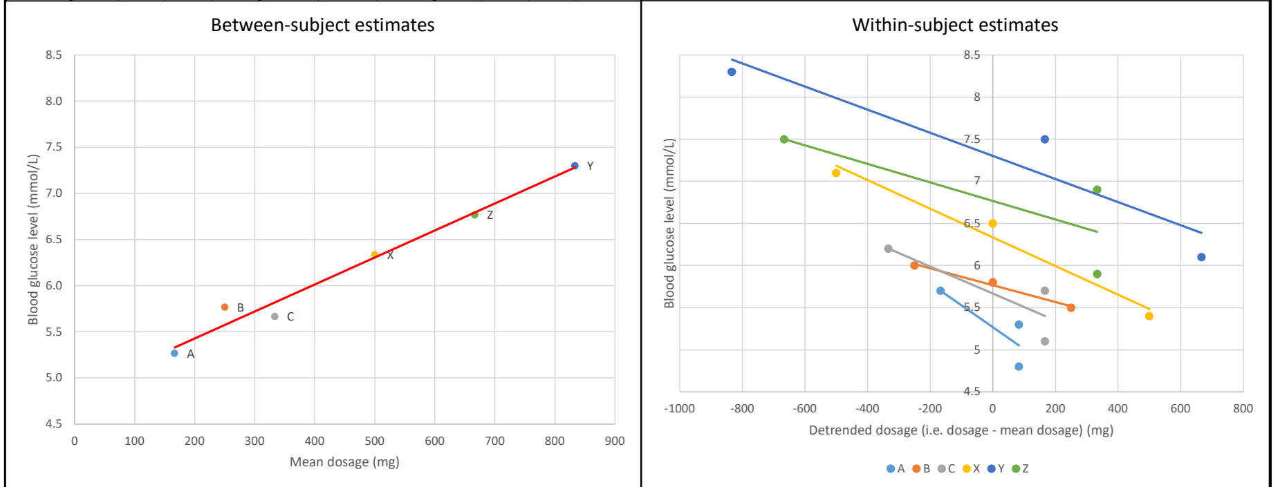
Fig. 1 A hypothetical example to illustrate the concept of the between-subject and the within-subject estimates.
