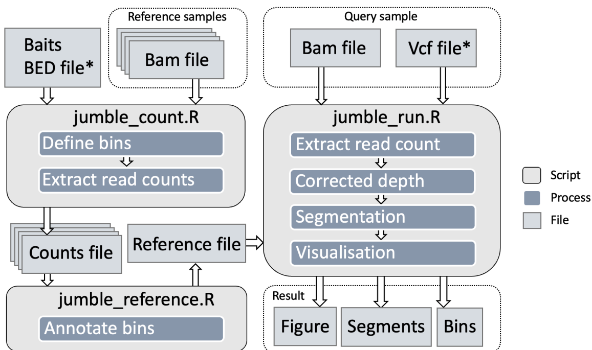
Supplementary Figure 1. Schematic of the Jumble computational tool architecture. Executable R scripts are run to process the reference and query samples. For a query sample, the main output consists of a figure file and two text files with tables of bins and segments. Asterisk indicates optional input.
