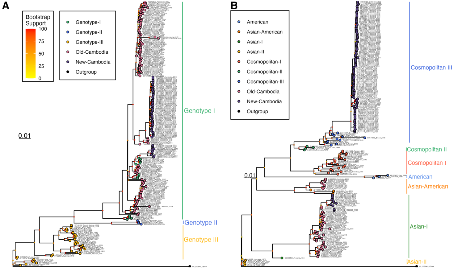
Fig. S18. Maximum likelihood phylogenetic tree constructed in RAxML (31) to illustrate how newly-contributed A DENV-1 and B DENV-2 sequences relate to all known genotypes of the corresponding serotype. Tips are colored by genotype within each serotype, with our Cambodia sequences highlighted in pink and historical Cambodia sequences available in GenBank depicted in purple. Clade bars highlight the extent of each genotype. Trees were constructed using a GTR+I+G4 nucleotide substitution model and rooted in DENV-4 (accession number NC_002640).
