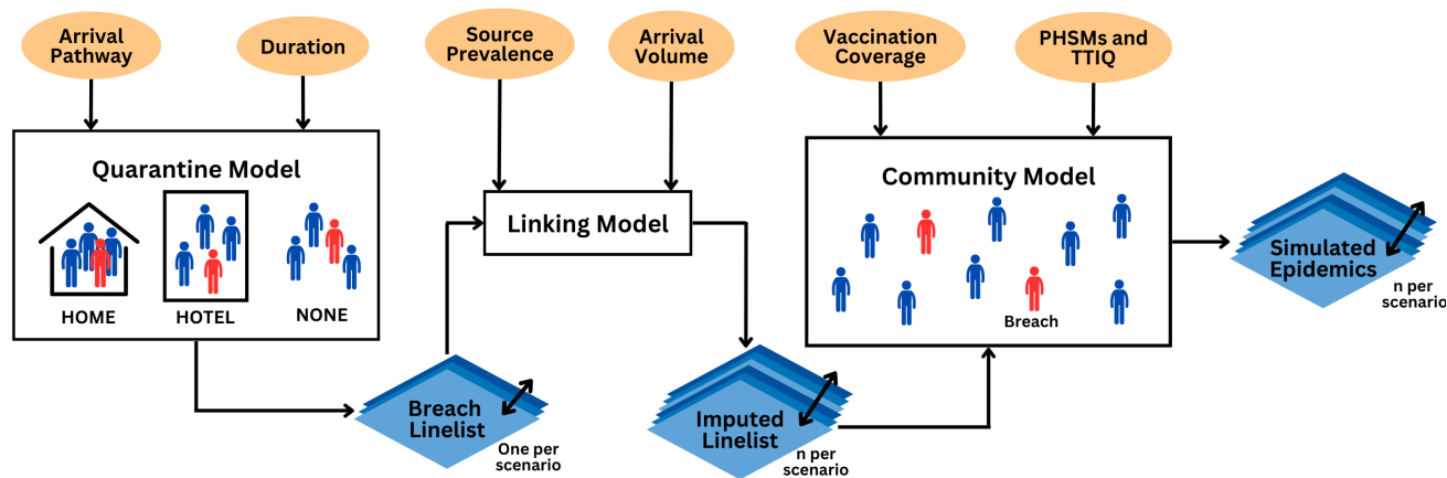
Fig 1. Schematic depicting the modelling framework used in this analysis. An individual-based model of the quarantine system, exploring quarantine pathway, duration and testing, is implemented to generate characteristics of breach events resulting from travellers and workers. A linelist of breach events, containing individual-level characteristics, for each scenario is generated from the quarantine model. These breach events are subsequently sampled appropriately given travel volumes and source prevalence to generate multiple linelists of breach events for each scenario, including the time the breach enters the community. Community characteristics, such as level of public health and social measures (PHSMs), test-trace-isolate-quarantine (TTIQ) system effectiveness, and age-specific vaccination coverage are implemented in the community model where breaches are introduced and subsequent outbreaks can be simulated for each breach linelist.
