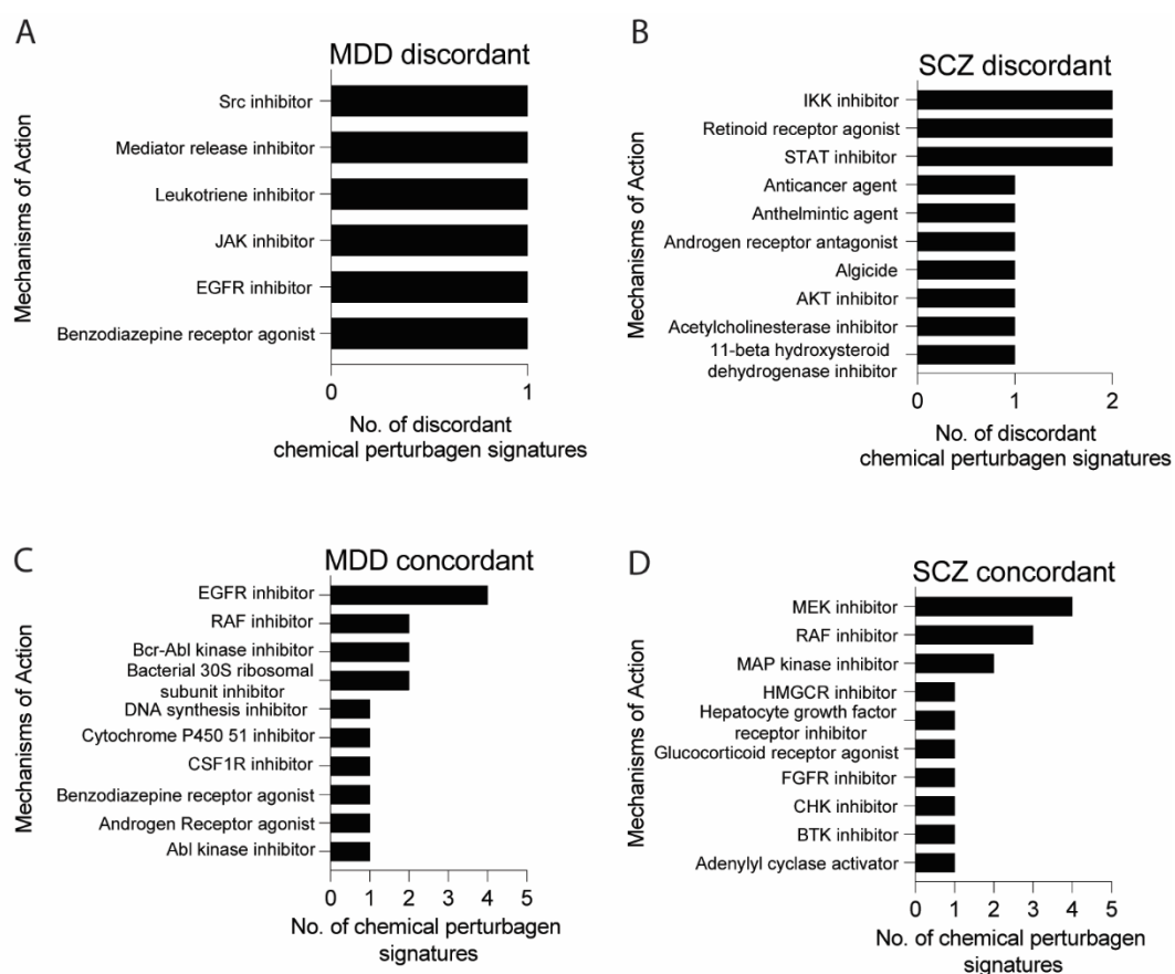
Fig S3. LINC analysis MDD and SCZ. The mechanisms of action (MOA) of the chemical perturbagens with LINC signatures that are discordant (dissimilar) to the MDD (A) and SCZ (B) disease signatures or concordant (similar) to the MDD (C) and SCZ (D) disease signatures. MDD major depressive disorder, MOA mechanism of action, SCZ schizophrenia.
