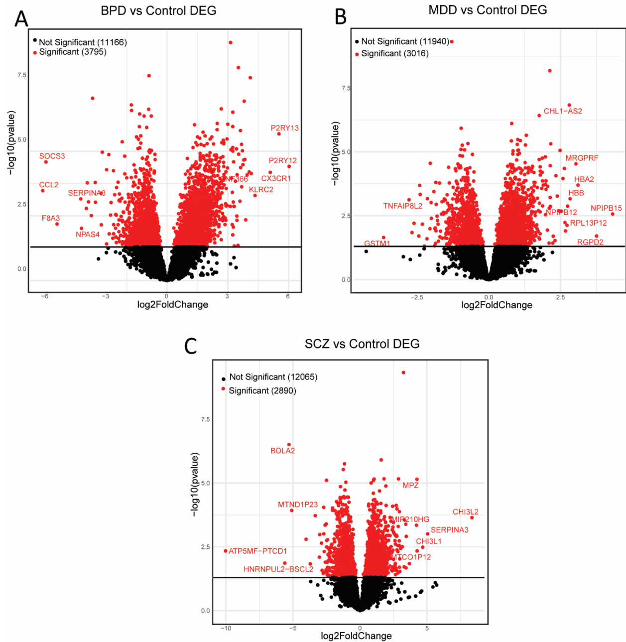
Fig S1. Volcano Plot. Volcano plot of -\log_{10}(\text{p-value}) (y-axis) and \log_2 fold change (x-axis) of differentially expressed gene transcripts in BPD (A), MDD (B) and SCZ (C). Significant genes are indicated by red dots, above the horizontal line indicating significance threshold ( -\log_{10}(\text{p}<0.05) ). Top differentially expressed genes (DEGs) are named on each figure. BPD bipolar disorder, MDD major depressive disorder, SCZ schizophrenia.
