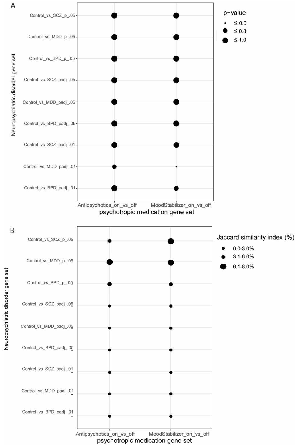
Fig S5. Psychotropic medication gene set enrichment. (A) Hypergeometric overlap analysis found no significant overlap ( p > 0.05 all comparisons) of BPD, MDD and SCZ DEGs
