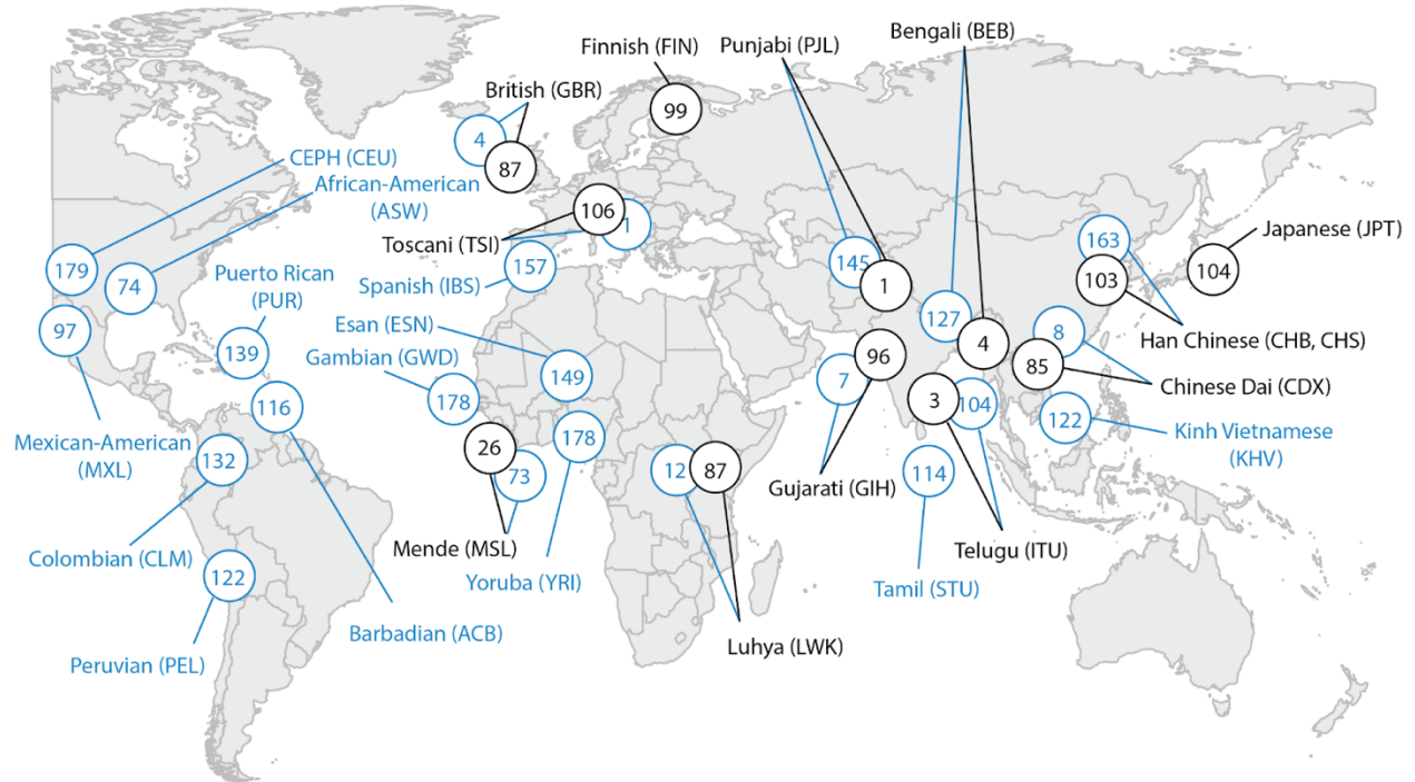
Supplementary Fig. 1 | Samples used as imputation targets (black) and reference (blue) in the 1000 Genomes 30x Dataset.
