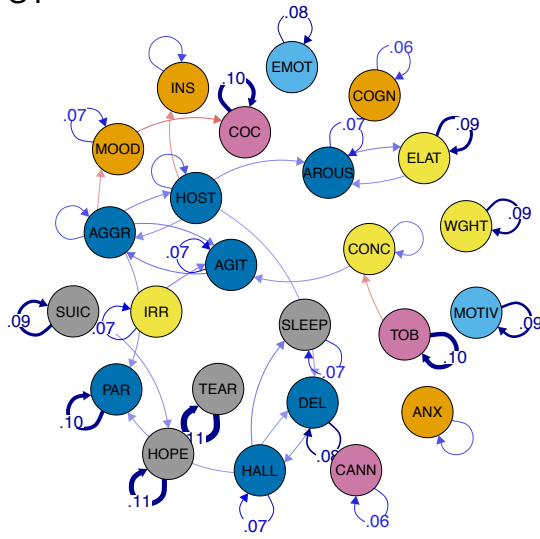
C. PSY
