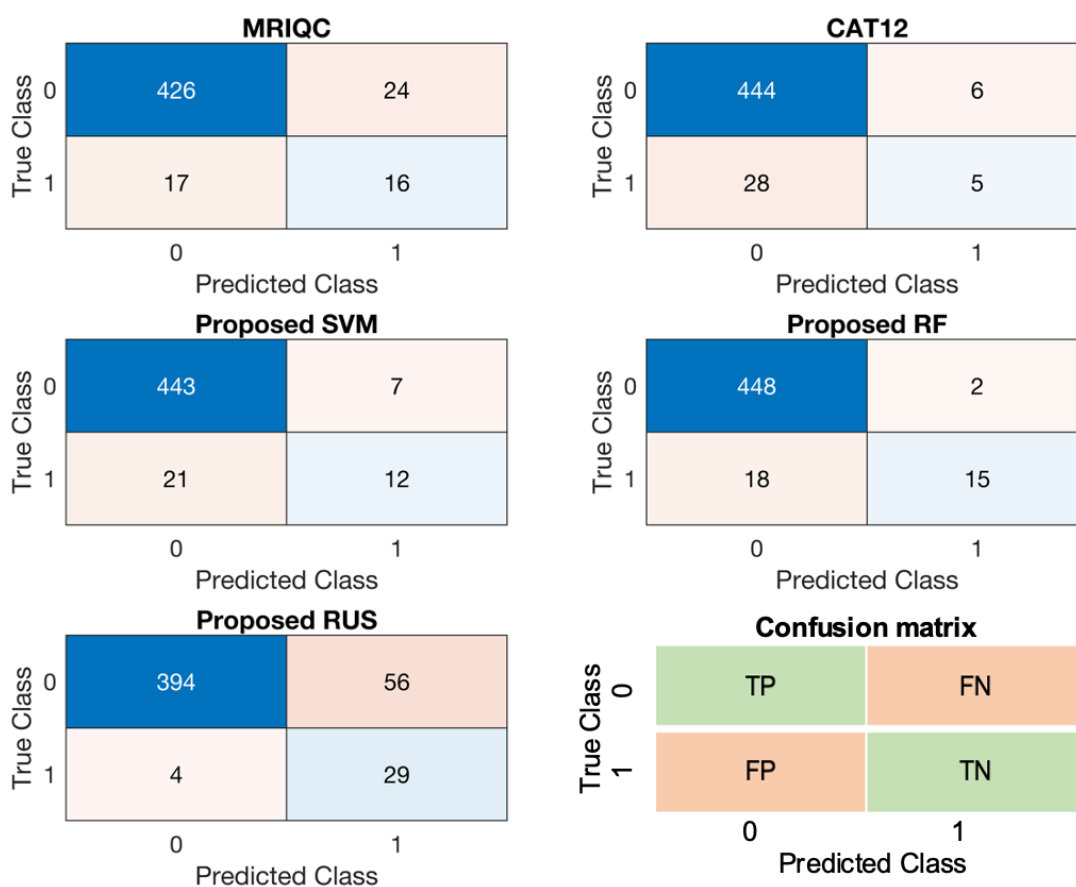
Figure S1. Confusion matrices showing total number of true positives, true negatives, false positives, and false negatives in the test data for MRIQC, CAT12 and proposed classifiers. Class 0 represents the accept class (positive), while class 1 represents the reject class (negative).
