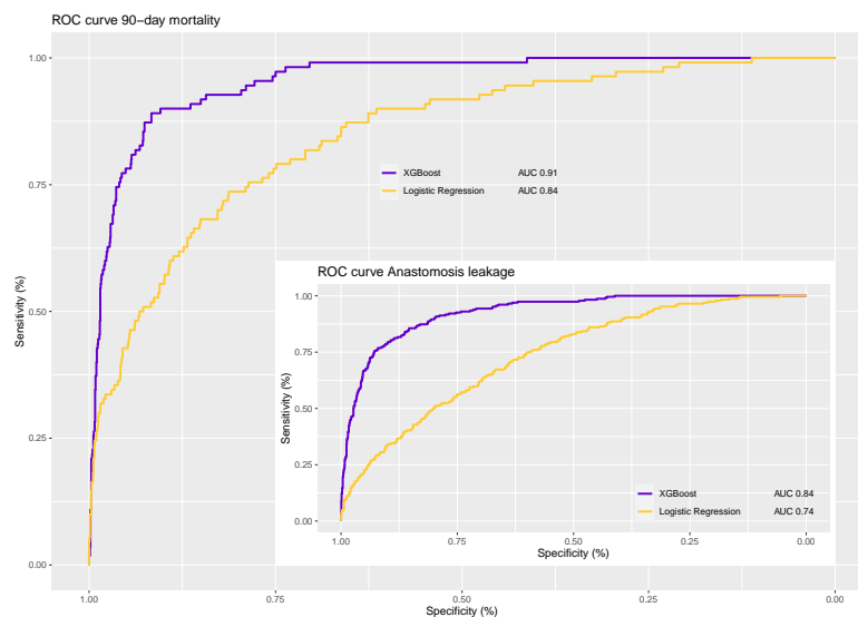
Fig. 1. Receiver operating characteristic (ROC) curves. Main: ROC curve 90-day mortality. Inset: ROC curve Anastomosis leakage
