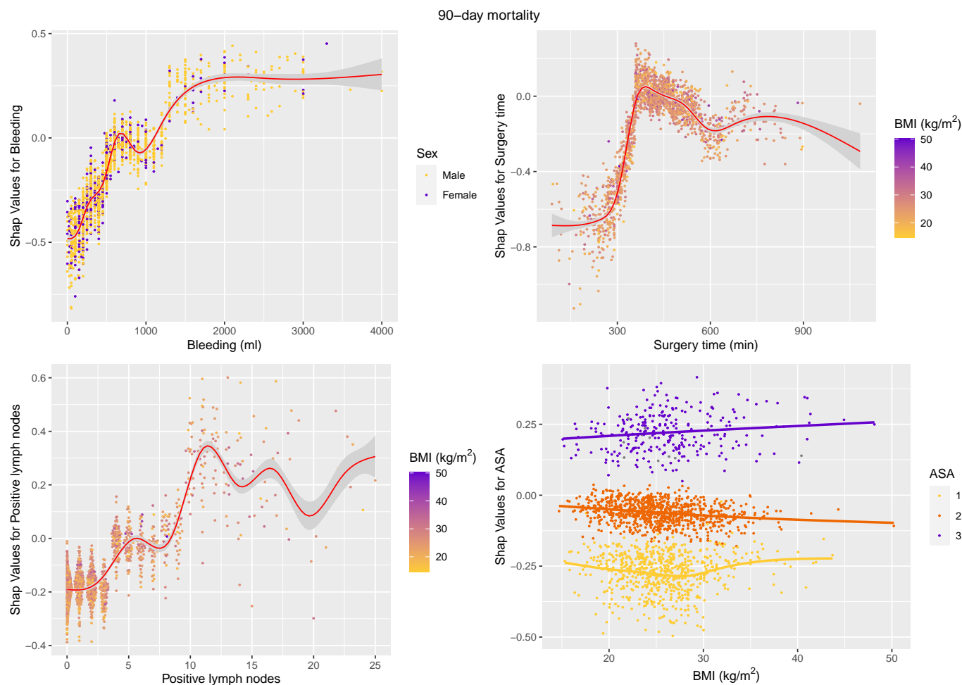
Fig. 5. SHAP values for 90-day mortality
