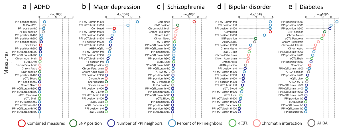
Figure 3. PPI-based mapping methods show the strongest correspondence between treatment targets and genes implicated in a GWAS for bipolar disorder and diabetes. Circles represent the significance of the association between the treatment-based score, s_{drug} , and GWAS-based score, s_{GWAS} , for a selected disorder. The significance is quantified using a permutation-based p-value comparing the empirical GWAS-treatment matching score \rho to a set of 5000 matching scores generated using a selection of random drugs [see details in eMethods 5 in Supplement 1]. The position of the circle corresponds to -\log_{10}(p) where higher values indicate a more significant association. Subplots correspond to different disorders: (a) ADHD, (b) major depression, (c) schizophrenia, (d) bipolar disorder, and (e) diabetes. Colors indicate different types of mapping methods: SNP position (dark green); spatial transcriptomic similarity (gray); chromatin interaction, Hi-c (pink); PPI network quantified as the proportion of neighbors (light blue); PPI network quantified as the total number of neighbors (dark blue); and eQTL (light green); linear combination of all measures (red); the null model was also adjusted to incorporate the linear regression across all measures in each iteration to account for this optimization step). Horizontal lines represent the degree of statistical significance: light gray line – p^{perm} = 8.3 \times 10^{-3} (Bonferroni correction for six types of measures, this threshold provides guidance for the expected significance level considering that groups of measures derived from the same type of mapping method show a degree of similarity); dark gray line -- p^{perm} = 1.9 \times 10^{-3} (Bonferroni correction for 27 measures); black line -- p^{perm} = 3.7 \times 10^{-4} (Bonferroni correction for 27 measures and 5 disorders, this threshold provides guidance for a highly conservative correction assuming independence among all mapping methods and disorders). Permutation-based approach estimates a p-value with a minimum resolution of 2 \times 10^{-4} (corresponding to 1/5000). If the estimated p-value is lower, we conservatively place it at 2 \times 10^{-4} .
