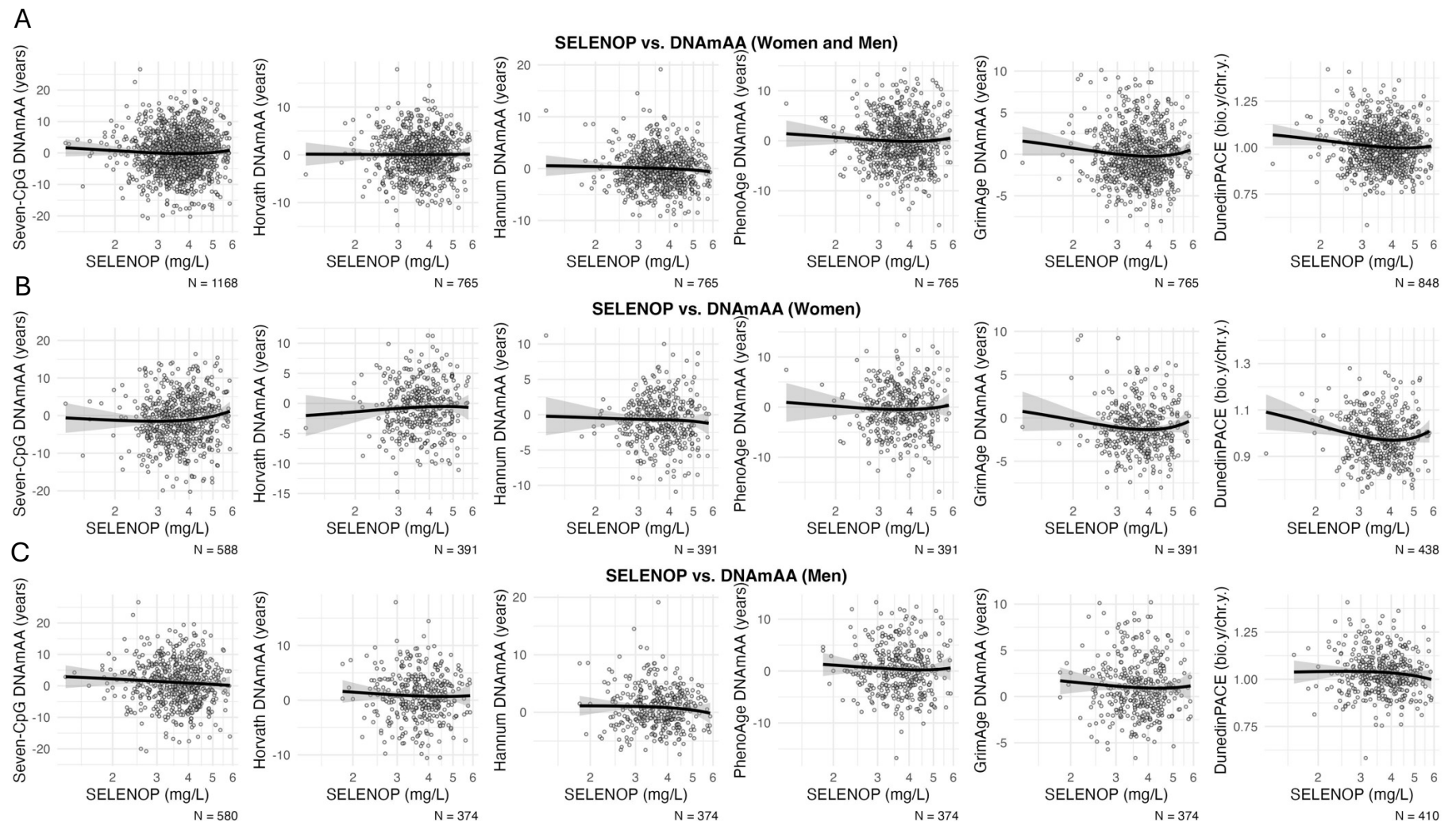
Supplementary Figure 3: Scatterplots of selenoprotein P levels and biological age estimators calculated from all six available epigenetic clocks in women and men (A) as well as in the all-women (B) and all-men (C) subgroup. The x-axis is log-scaled. All available participants of the older age group are included.
