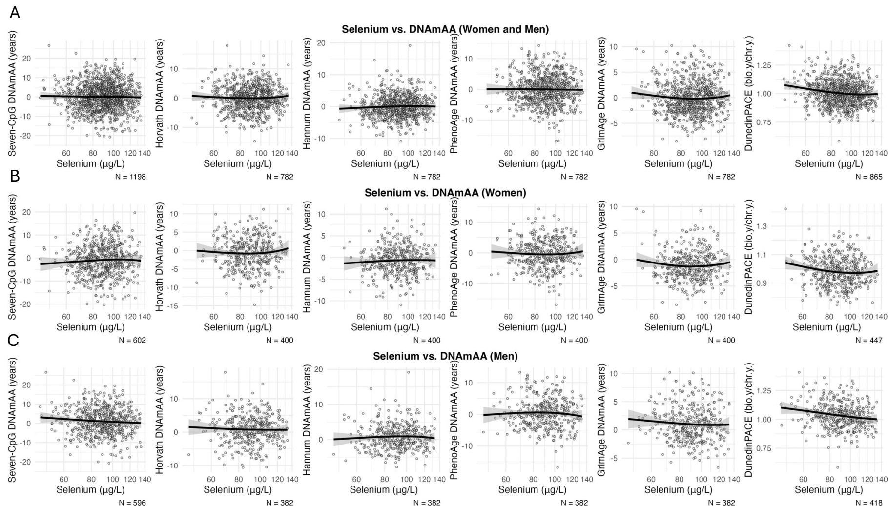
Supplementary Figure 1: Scatterplots of serum selenium levels and biological age estimators calculated from all six available epigenetic clocks in women and men (A) as well as in the all-women (B) and all-men (C) subgroup. The x-axis is log-scaled. All available participants of the older age group are included.
