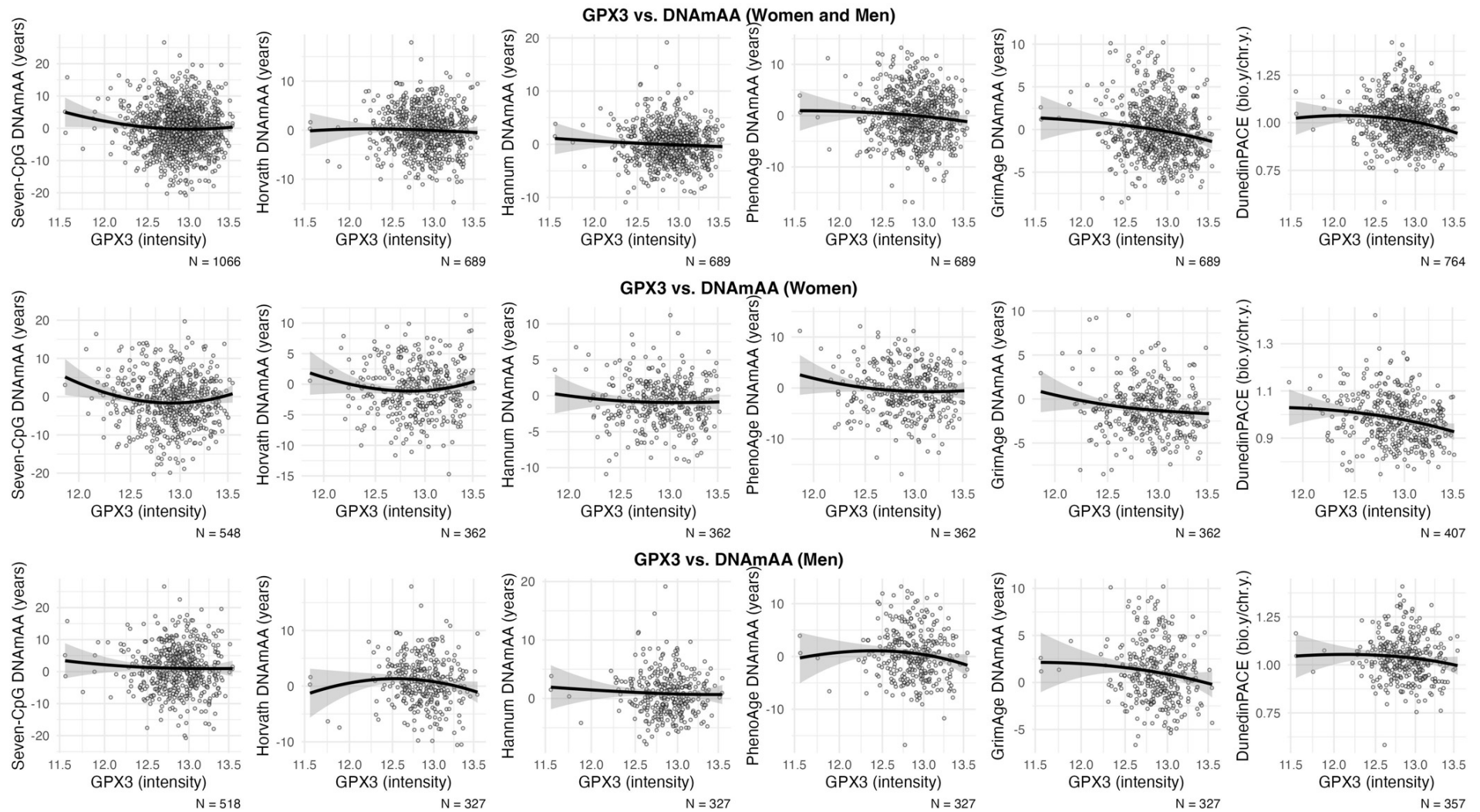
Supplementary Figure 3: Scatterplots of GPx3 intensity and biological age estimators calculated from all six available epigenetic clocks in women and men (A) as well as in the all-women (B) and all-me (C) subgroup. The x-axis is log-scaled. All available participants of the older age group are included.
