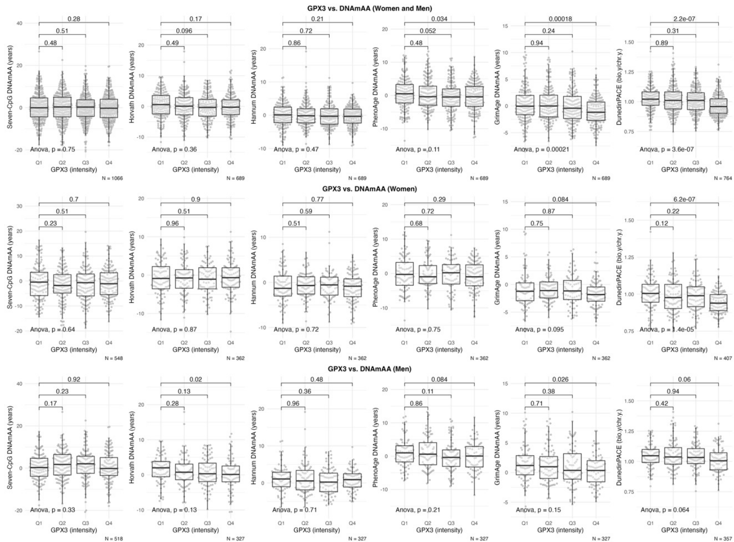
Supplementary Table 4: Boxplots of biological age estimators calculated by all six available epigenetic clocks stratified by quartiles of GPX3 intensities (proteomics) in men and women (A), women (B) and men (C). Statistical significance of difference between group means was assessed by t-test.
