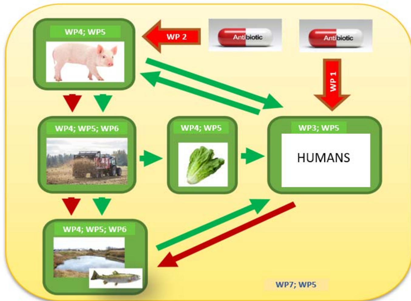
Figure 2. Development and spread of antibiotic resistance in relation to the work packages (WP) of the AMR-RITA project. The red arrows indicate the consumption of antibiotics and the transmission routes of antibiotic residues. Green arrows indicate transmission pathways of antibiotic-resistant bacteria and resistance genes.
