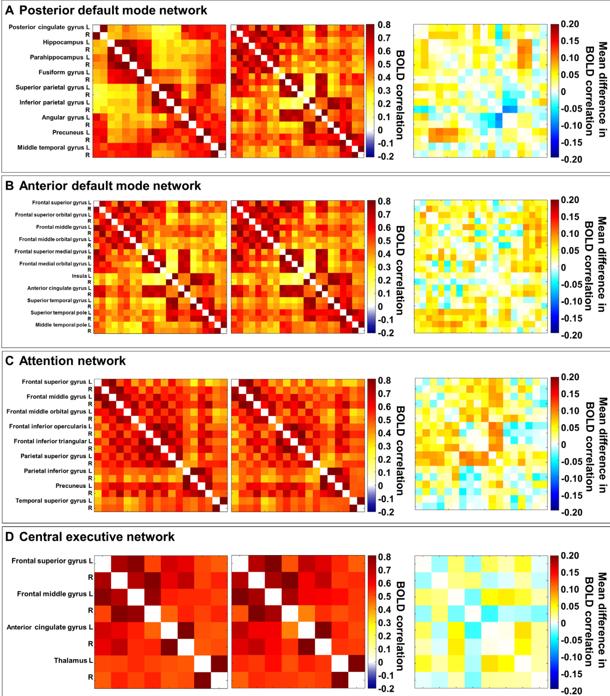
Figure S5: Functional connectivity matrices scaled by BOLD correlations indicated by resting-state functional MRI in the (A) posterior (pDMN) and (B) anterior default mode networks (aDMN), (C) attention network (AN), and (D) central executive control network (CEN) with the mean connectivity for individuals with (i) low blast exposure and (ii) high blast exposure, and (iii) the group difference. There were no blast-related differences in
