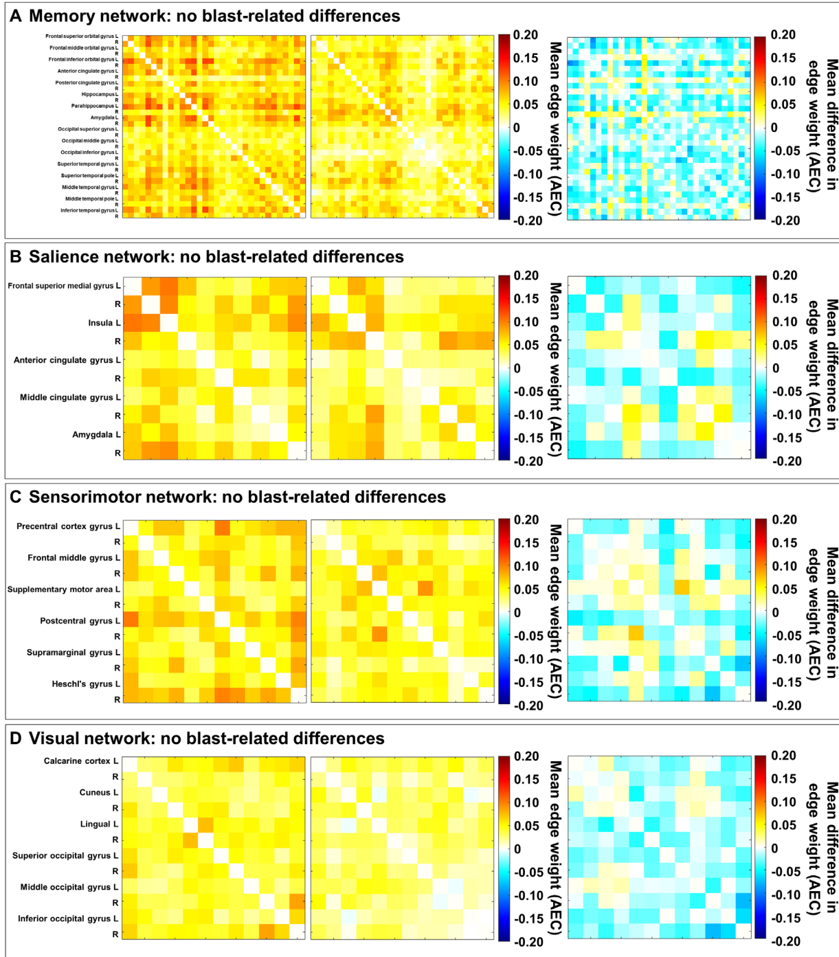
Figure S2: Functional connectivity matrices scaled by mean edge weight (AEC) measured by resting-state magnetoencephalography (MEG) at low gamma (30-55 Hz) range in the (A) memory network (MN), (B) salience network (SN), (C) sensorimotor network (SMN), and (D) visual network (VN) with the mean connectivity for individuals with (i) low blast exposure and (ii) high blast exposure, and (iii) the group difference.
