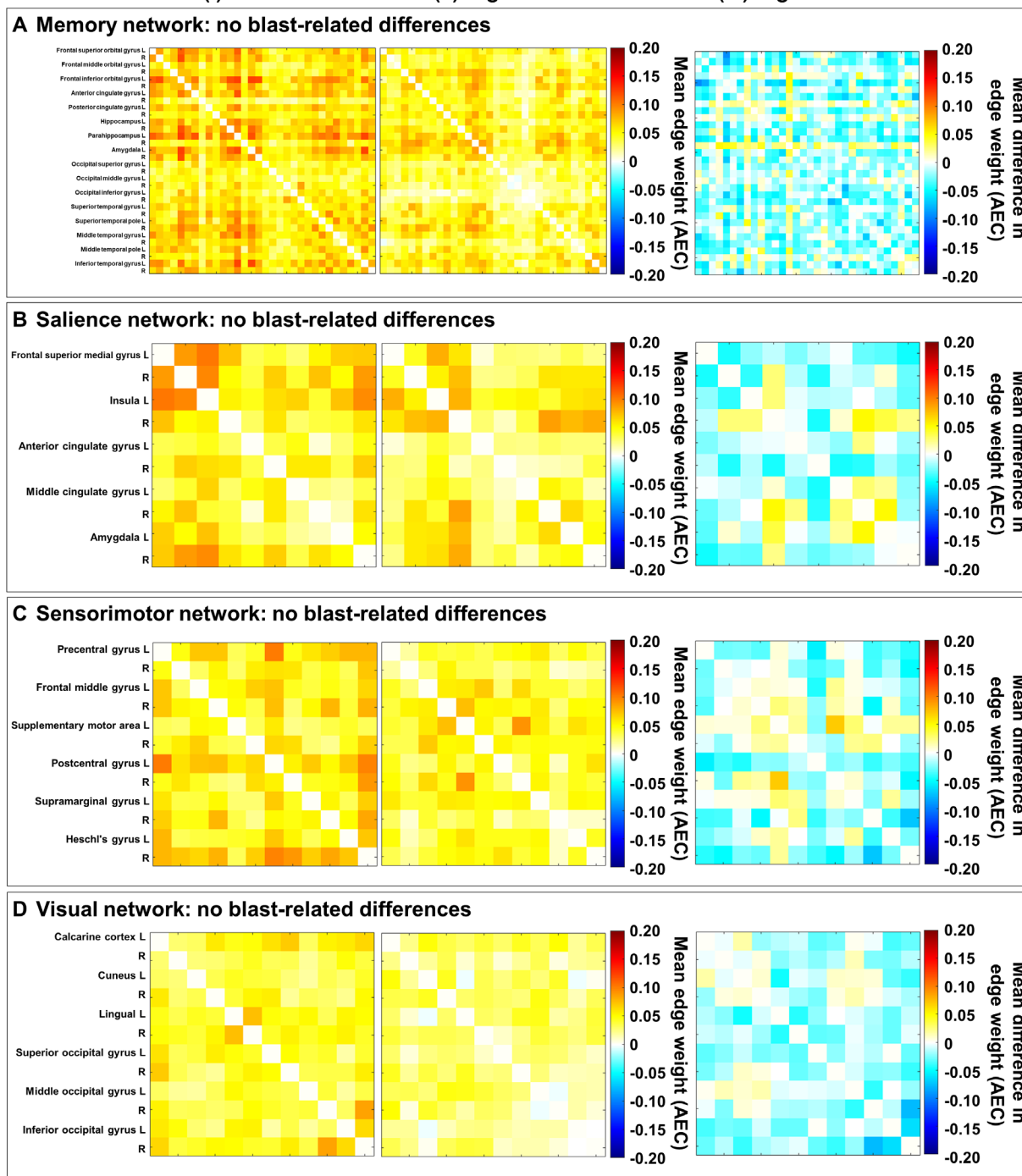
Figure S4: Functional connectivity matrices scaled by mean edge weight (AEC) measured by resting-state magnetoencephalography (MEG) at high gamma (80-150 Hz) range in the (A) memory network (MN), (B) salience network (SN), (C) sensorimotor network (SMN), and (D) visual network (VN) with the mean connectivity for individuals with (i) low blast exposure and (ii) high blast exposure, and (iii) the group difference.
