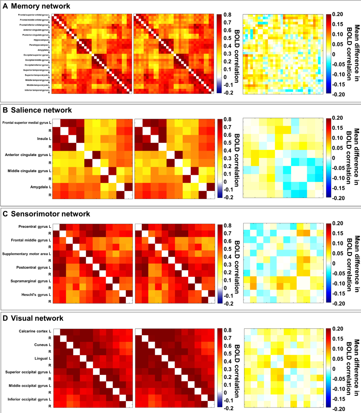
Figure S6: Functional connectivity matrices scaled by BOLD correlations indicated by resting-state functional MRI in the (A) memory network (MN), (B) salience network (SN), (C) sensorimotor network (SMN), and (D) visual network (VN) with the mean connectivity for individuals with (i) low blast exposure and (ii) high blast exposure, and (iii) the group difference. There were no blast-related differences in (A) MN, (B) SN, (C) SMN, or (D) VN
