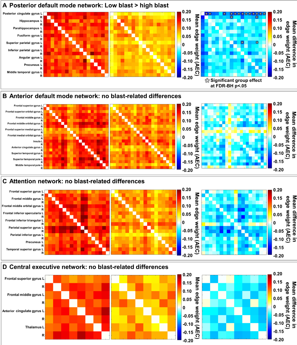
Figure S3: Functional connectivity matrices scaled by mean edge weight (AEC) measured by resting-state magnetoencephalography (MEG) at high gamma (80-150 Hz) range in the (A) posterior (pDMN) and (B) anterior default mode networks (aDMN), (C) attention network (AN), and (D) central executive control network (CEN) with the mean connectivity for individuals with (i) low blast exposure and (ii) high blast exposure, and
