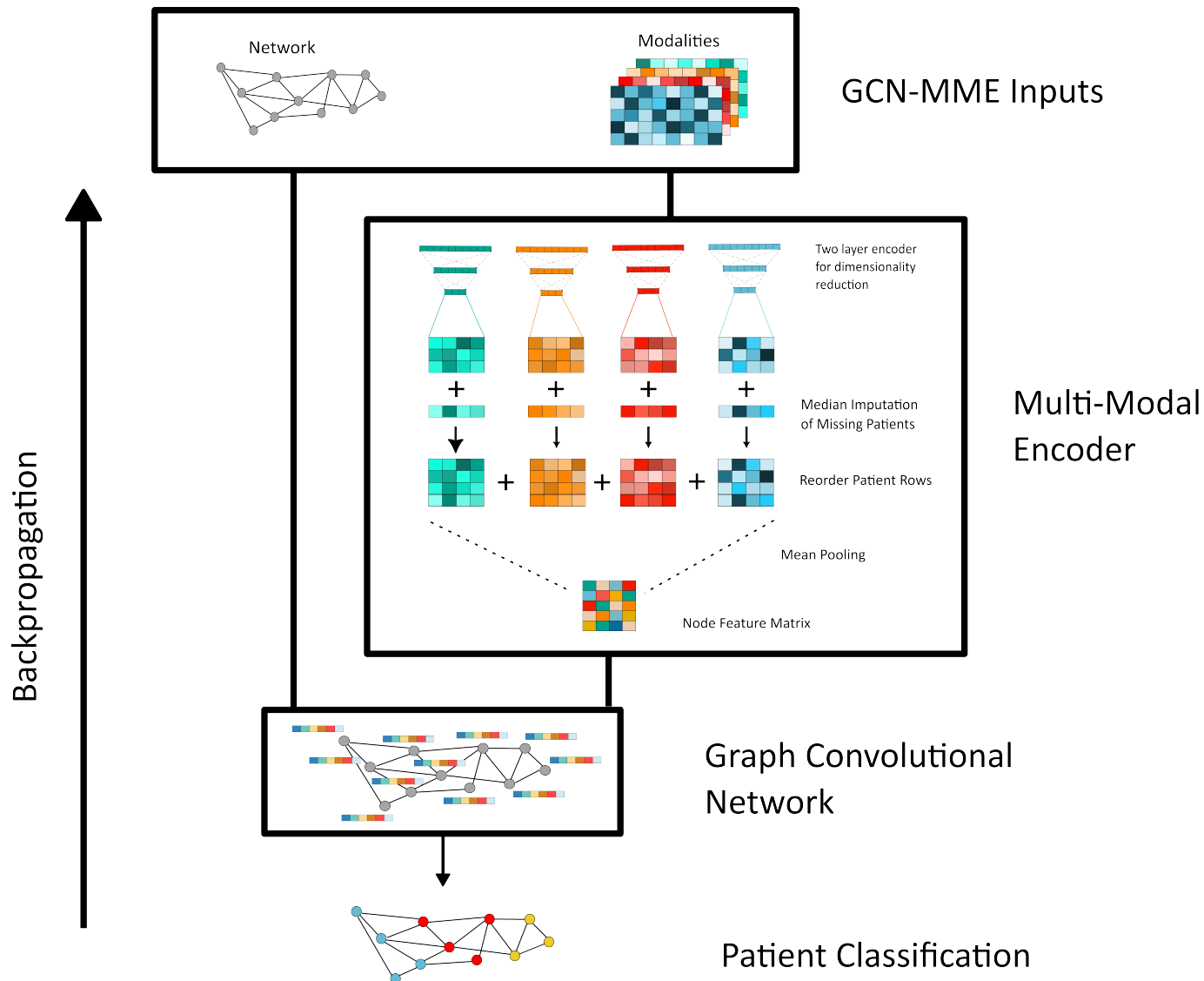
Figure 1. Graph Convolutional Network - Multi-Modal Encoder Architecture (GCN-MME) | The GCN-MME takes as input a fixed network and any number of modalities. The nodes in the network correspond to patients, and each patient is present in at least one modality. The modalities are encoded for dimensionality reduction using a two layer encoder. After the second layer, median imputation is performed to include patients missing from that modality but included in the network and at least one other modality. There is a shared latent embedding between the encoders, and the imputed second layers of each encoder are joined using mean pooling. This shared latent embedding forms the node features for the GCN. Patient classification is performed using the GCN with the loss back propagated through the entire GCN, thus, training each encoder in series with the GCN.
