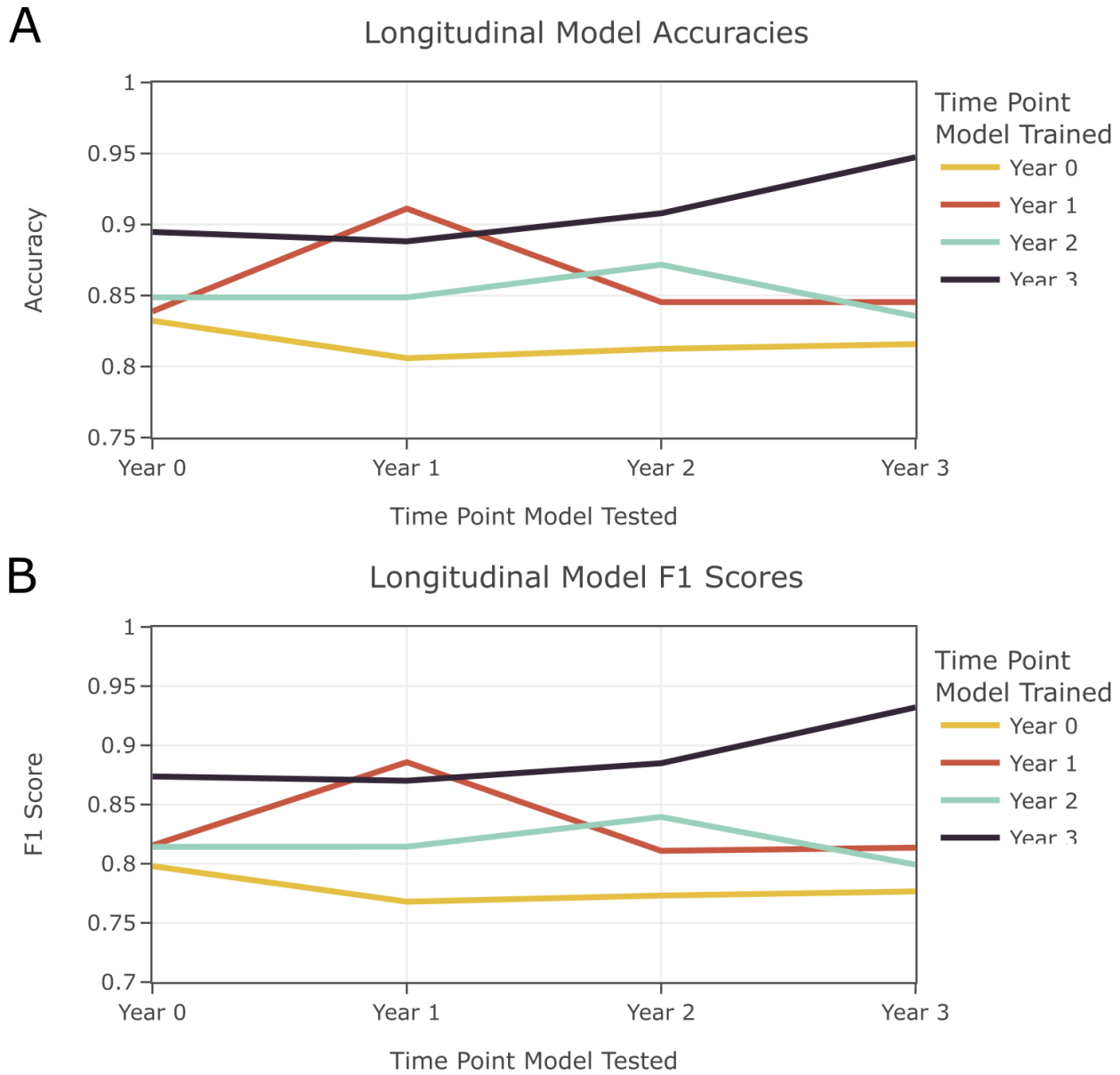
Figure 4. The performance metrics in the longitudinal experiment when models were trained at each time point and tested at all time points
