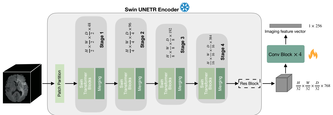
Figure S4: Image feature extraction. The Swin UNETR encoder, utilizing pre-trained weights, was leveraged to extract image embeddings from multi-sequence MRI scans into a latent space representation. Subsequently, these embeddings underwent a series of downsampling convolutional operations to achieve a condensed token dimension of 1 \times 256 . This dimensional reduction facilitated a consistent input format for both imaging and non-imaging data into the backbone transformer. Within this architecture, the Swin UNETR encoder’s weights remained static (frozen), ensuring the integrity of the pre-trained features, while the downsampling blocks were subject to optimization during the training phase, allowing for adaptive learning of the imaging feature vector.
