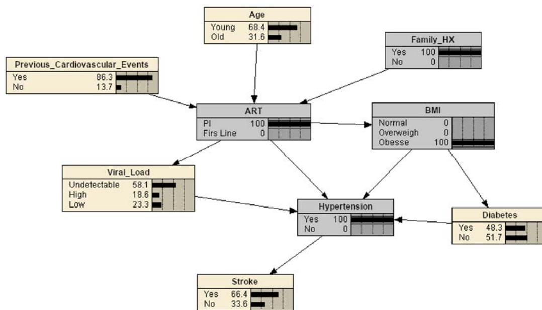
Figure 2: Bayesian reasoning for Stroke prediction when the evidence variables are ART, Hypertension, Family history of Stroke and BMI
