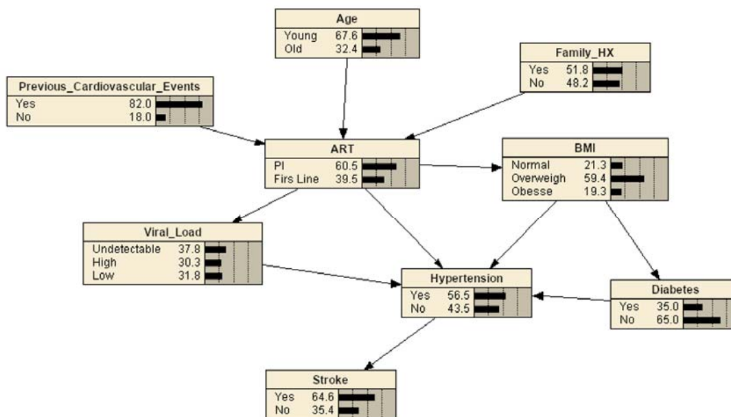
Figure 1/ Bayesian network for predicting Stroke with available risk factors. The tree-augmented Bayesian network used 9 variables selected by the wrapper of the Bayesian network for prediction
