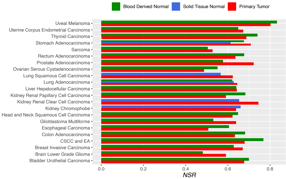
Fig 7. The comparisons of NSR (normalized stochasticity ratio) between PT (primary tumor), SN (solid tissue normal) and blood derived normal (B) for various cancer types with WGS datasets.
