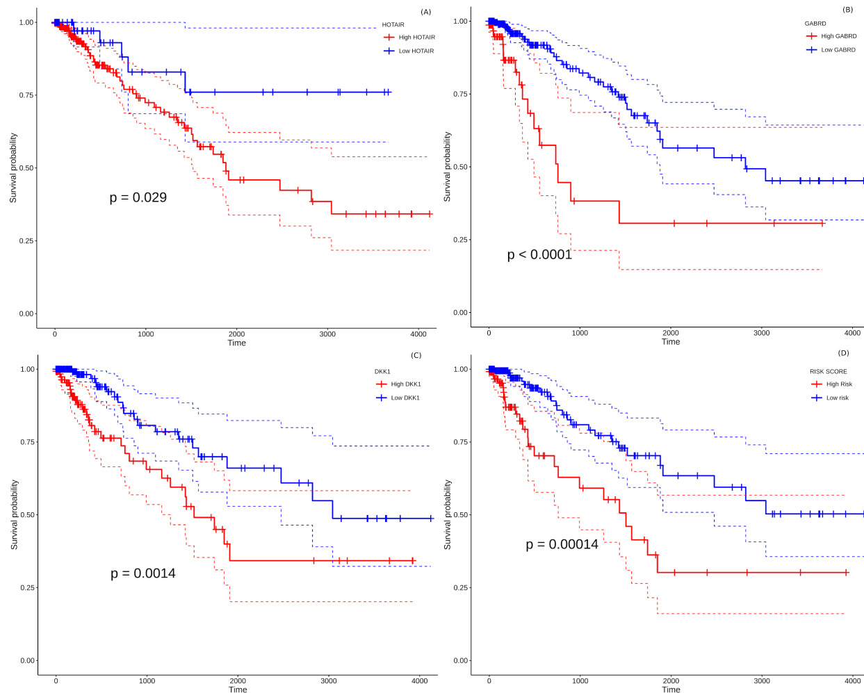
Fig 9. Survival analysis of prognostically significant stage-salient genes. Univariate Cox regression analysis of (A) HOTAIR, (B) GABRD, (C) DKK1; and (D) construction of optimal multivariate panel comprising the above biomarkers. Over-expression of the prognostic biomarkers has a significant effect on the survival probabilities ( P < 0.05 ), and elevates the patient risk. Red - high-risk, blue - low-risk; colored dashed lines represent corresponding 95% confidence intervals.
