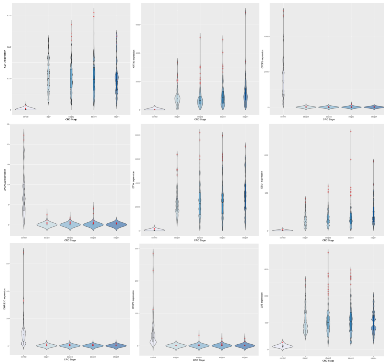
Fig 3. Expression trends of the top 9 DEGs from the linear modeling. Row-wise: CDH3, KRT80, OTOP2, AADA2L2, ETV4, ESM1, DHRS7C, OTOP3, JUB. It can be observed that some genes are downregulated to near-zero expression as CRC progresses (notably OTOP2, OTOP3, AADA2L2 and DHRS7C).
