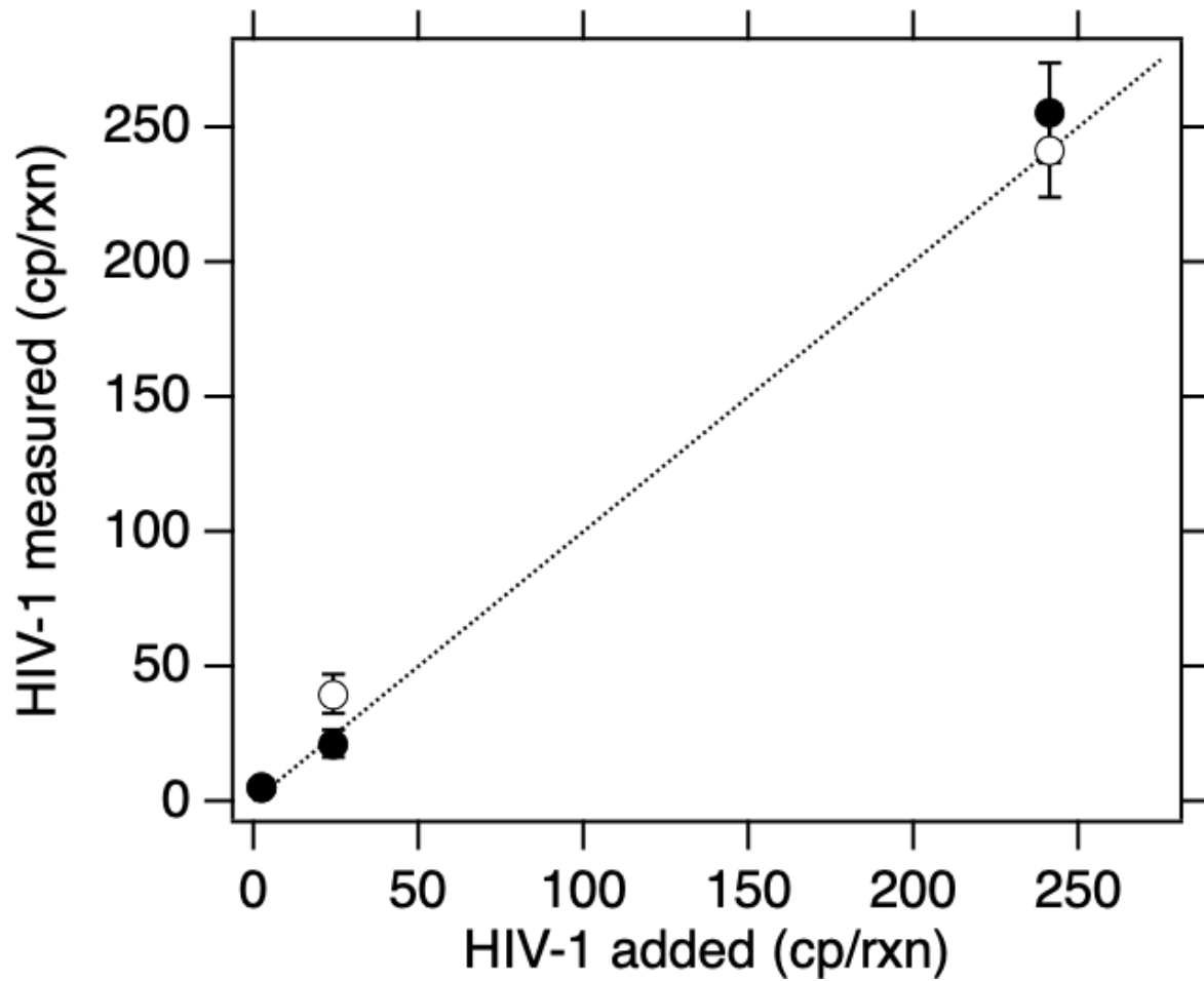
Figure S1. Multiplex assay performance. The concentration of the HIV-1 target in units of copies per reaction input and measured is provided. The white symbols are for reactions without the 7 background nucleic-acid targets and black symbols include high concentrations of the 7 other nucleic-acid targets. Error bars are standard deviations, if error bars cannot be seen, then they are smaller than the symbol. The line represents the 1:1 line.
