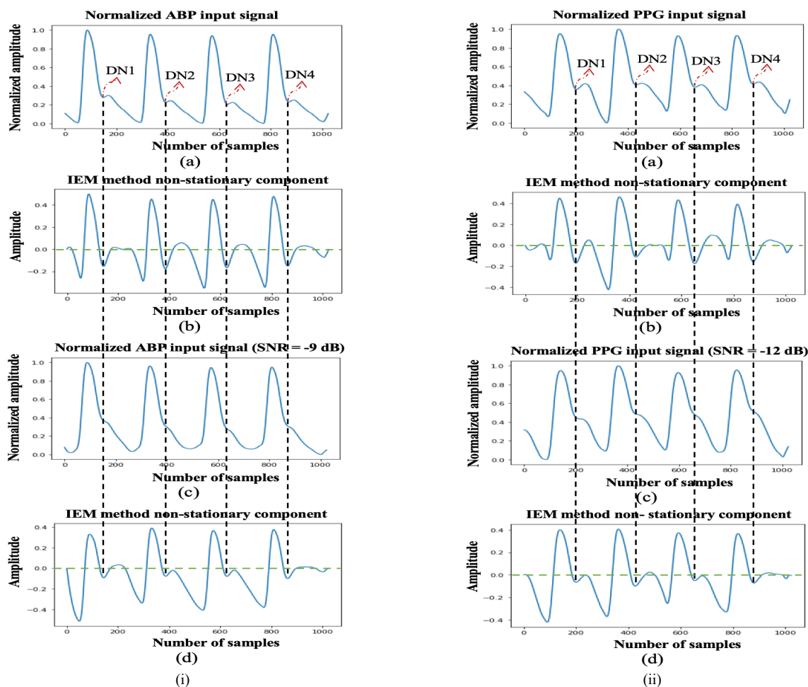
Fig. 9. (i) (a) Normalized ABP input signal with marked dicotic notch locations by an experienced researcher; (b) IEM method non-stationary component; (c) Normalized ABP input signal at SNR = -9 dB; (d) IEM method non-stationary component. (ii) ((a) Normalized PPG input signal with manually marked dicotic notches; (b) IEM method non-stationary component; (c) Normalized PPG input signal at SNR = -12 dB; (d) IEM method non-stationary component.
