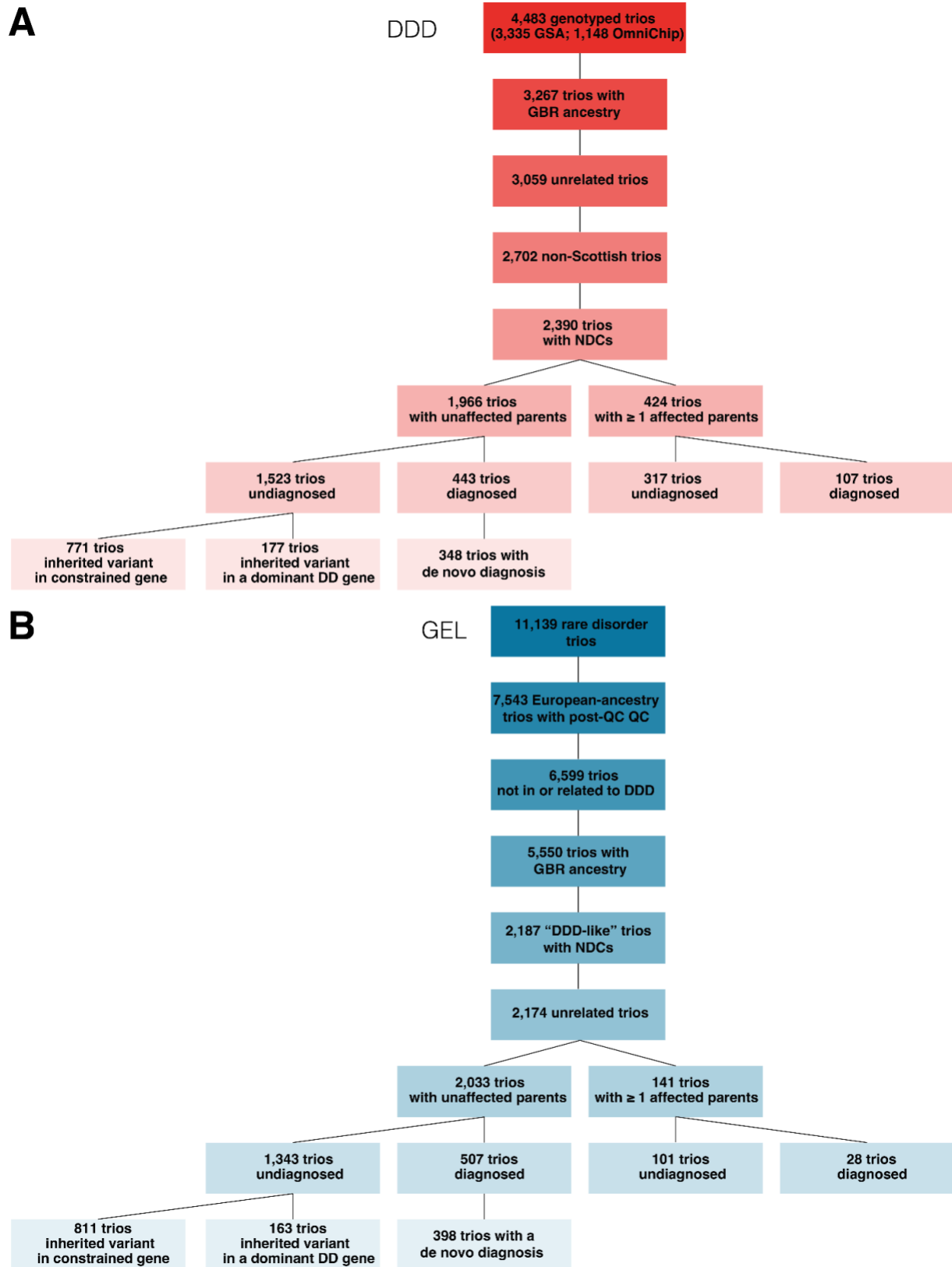
Supplementary Figure 16. Flow diagram of trio filtering in A) DDD and B) GEL.
