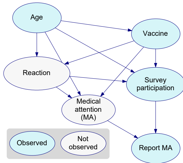
Figure 3: The simplified DAG. which depicts the relationship of a minimum set of variables required to investigate how biological, behavioural and procedural processes interact to influence the probability of a reported MA using PPA method. See the Table 1 for the definition of each variable, and see Supplementary Dictionary for how each variable is aligned with the full DAG.
