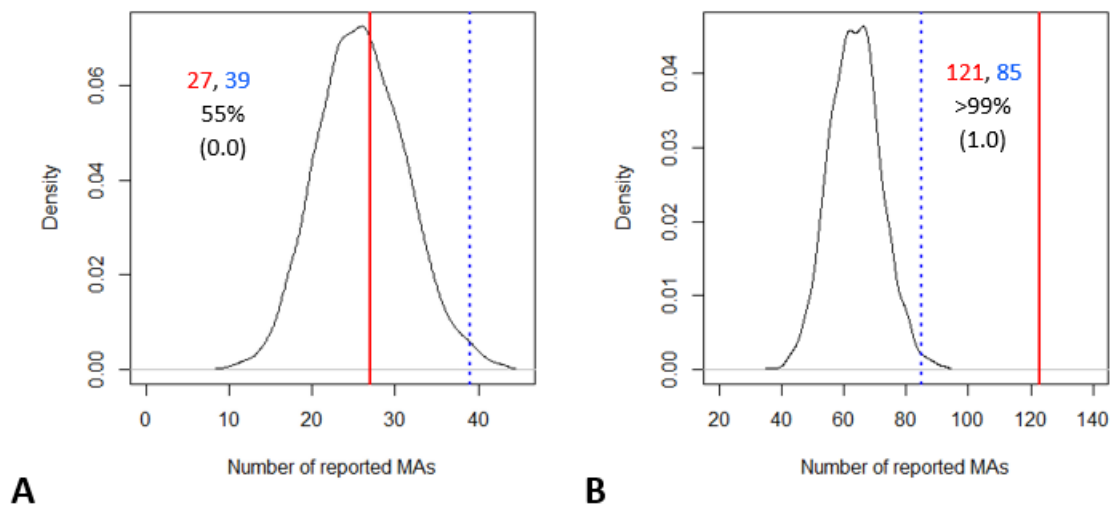
Figure 1: Illustrative outputs of the PPA method from a single simulation. The number of observed MAs, reported in red and the signal threshold reported in blue, are also indicated by the solid red lines and dotted blue lines, respectively. The percentile of the posterior predicted distribution is used here as an indication of distance of the number of reported MAs from the signal threshold. As the figure illustrates the outputs of just one simulation, the proportion of simulations with an alerted signal is 0.0 in Fig. 1A and 1.0 in Fig. 1B.
