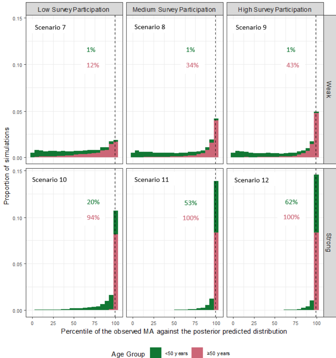
Figure 5: High Probability of Severe Reaction in Investigation Scenarios, Increase in biological processes compared to the reference scenario. Signals are flagged when the number of MAs exceeds the 99th centile (dotted lines). The proportion of simulations which generated a signal within each scenario are represented as percentages within each panel in this figure. See Table 1 and 2 for simulation parameters used in each scenario.
