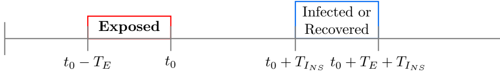
Fig 1: Initialization of the Exposed compartment. For an arbitrary but fixed t_0 , individuals who got exposed in the left shaded area (red) will get symptoms or recover in the right shaded area (blue).
