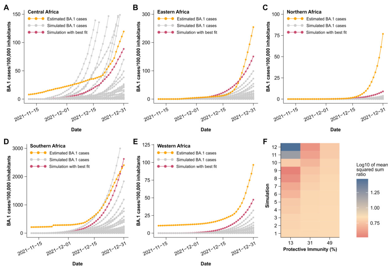
Figure 6: Simulation of Omicron/BA.1 cases.
