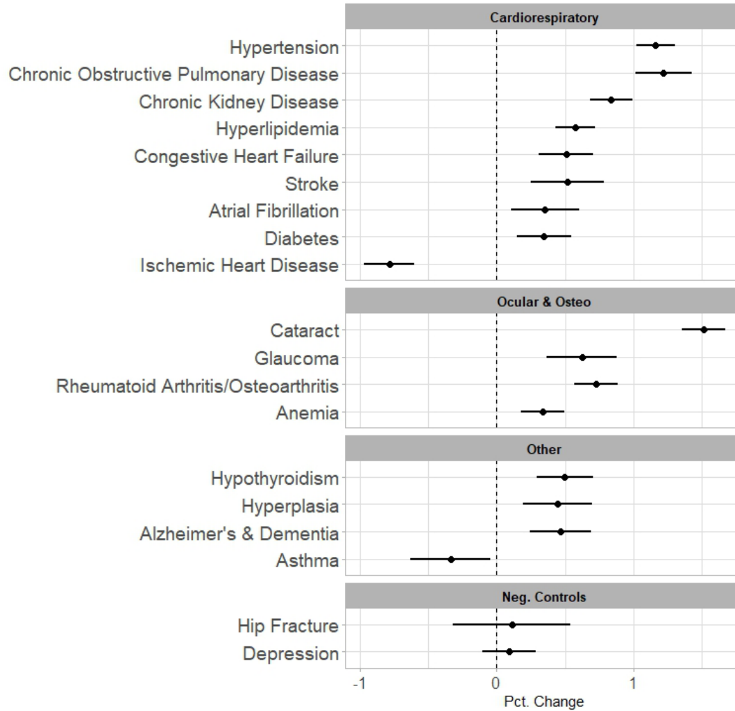
595 Figure 2. Estimated percent difference in incidence of 19 chronic health conditions for a 10 ng/L 596 increment in distance-weighted mean of per- and polyfluoroalkyl substances (PFAS) groundwater 597 concentration (and 95% confidence intervals) for final epidemiologic model: 1,696,247 Medicare 598 beneficiaries over age 65 living in California counties with more than 25% of drinking water from 599 groundwater, 2011-2017.
