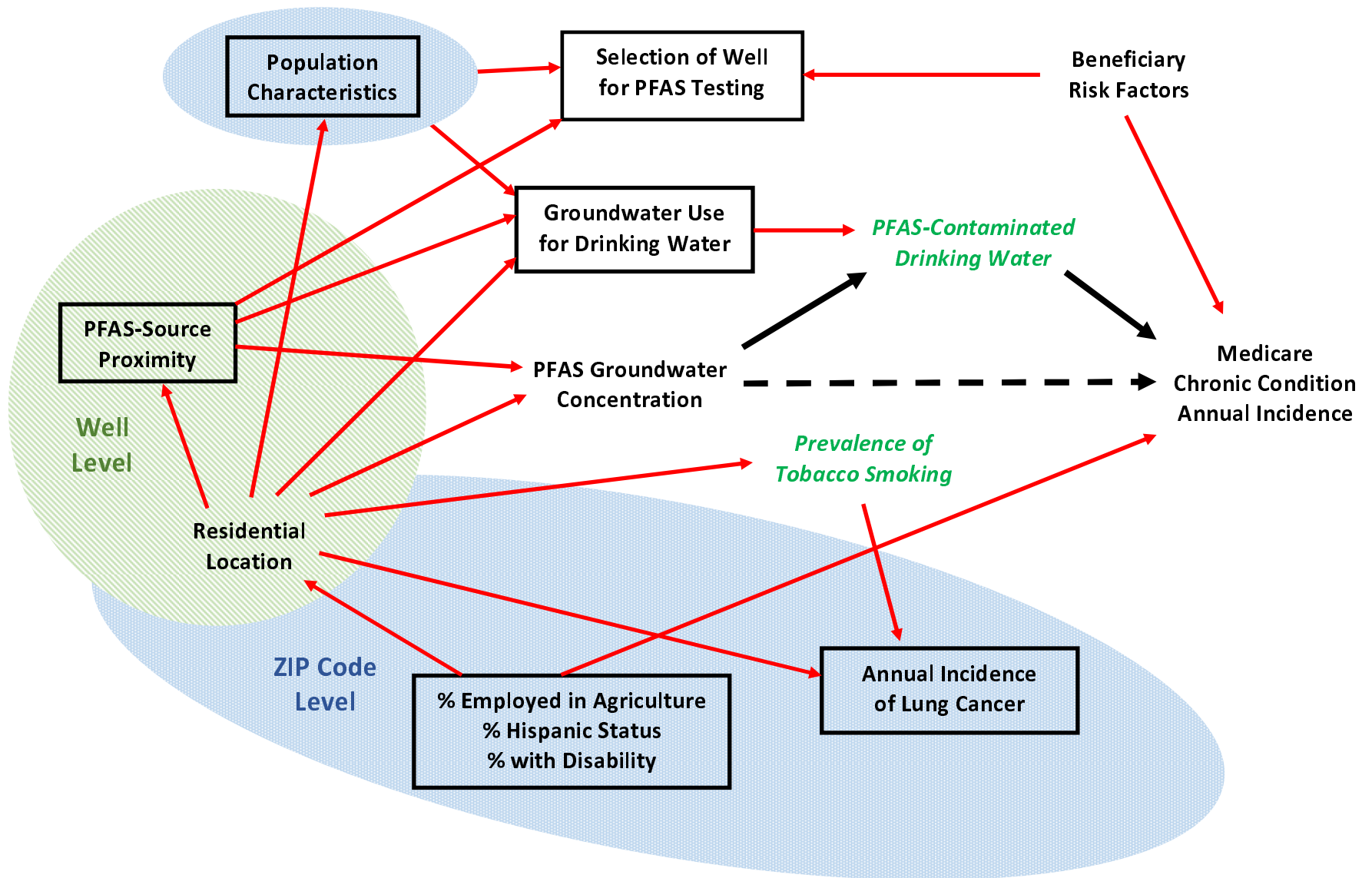
468 Figure S1. Directed Acyclic Graph (DAG) used for development of epidemiologic models.
