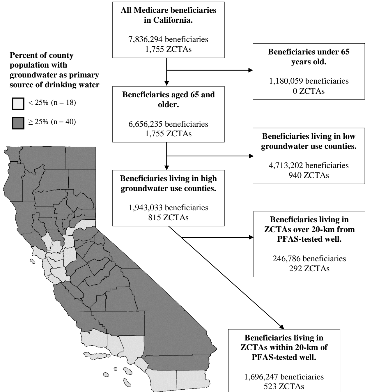
590 Figure 1. Flow diagram showing restrictions to cohort in number of Medicare beneficiaries and ZIP Code 591 Tabulation Areas (ZCTAs) with inset map of California counties showing proportion of population 592 supplied with drinking water derived from groundwater: 2011-2017.
