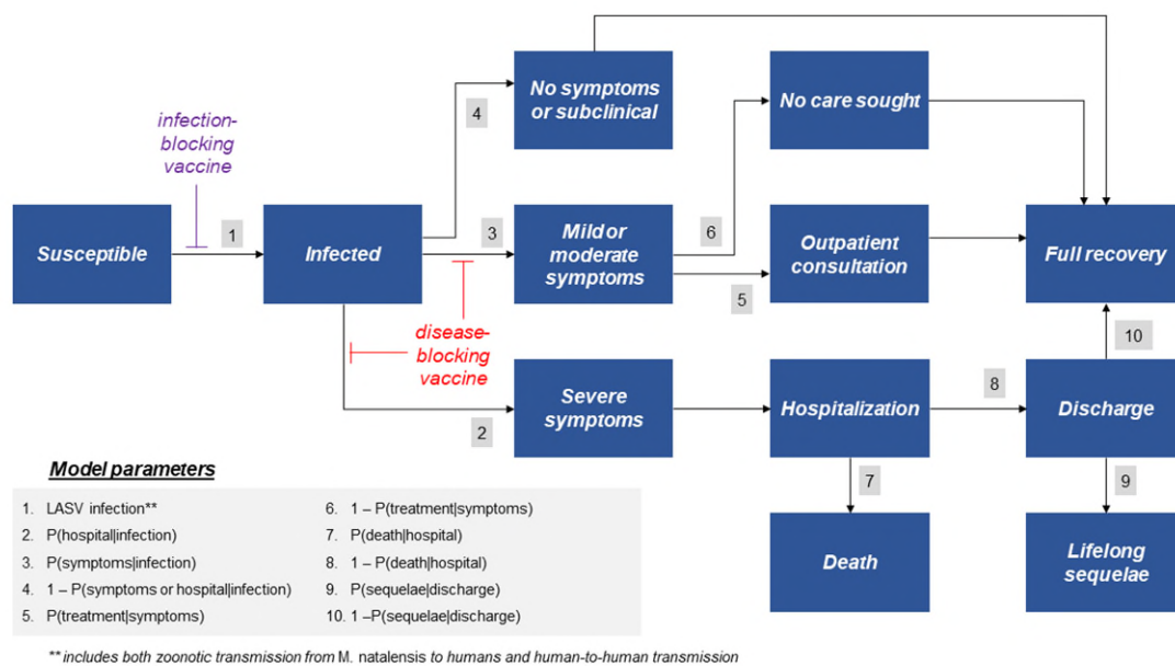
Figure C.1. Schematic of the health-economic model. Model parameters (transition probabilities) are described further in Table C.1 . Transition probabilities equal 1 for arrows with no parameter listed. LASV: Lassa virus.
