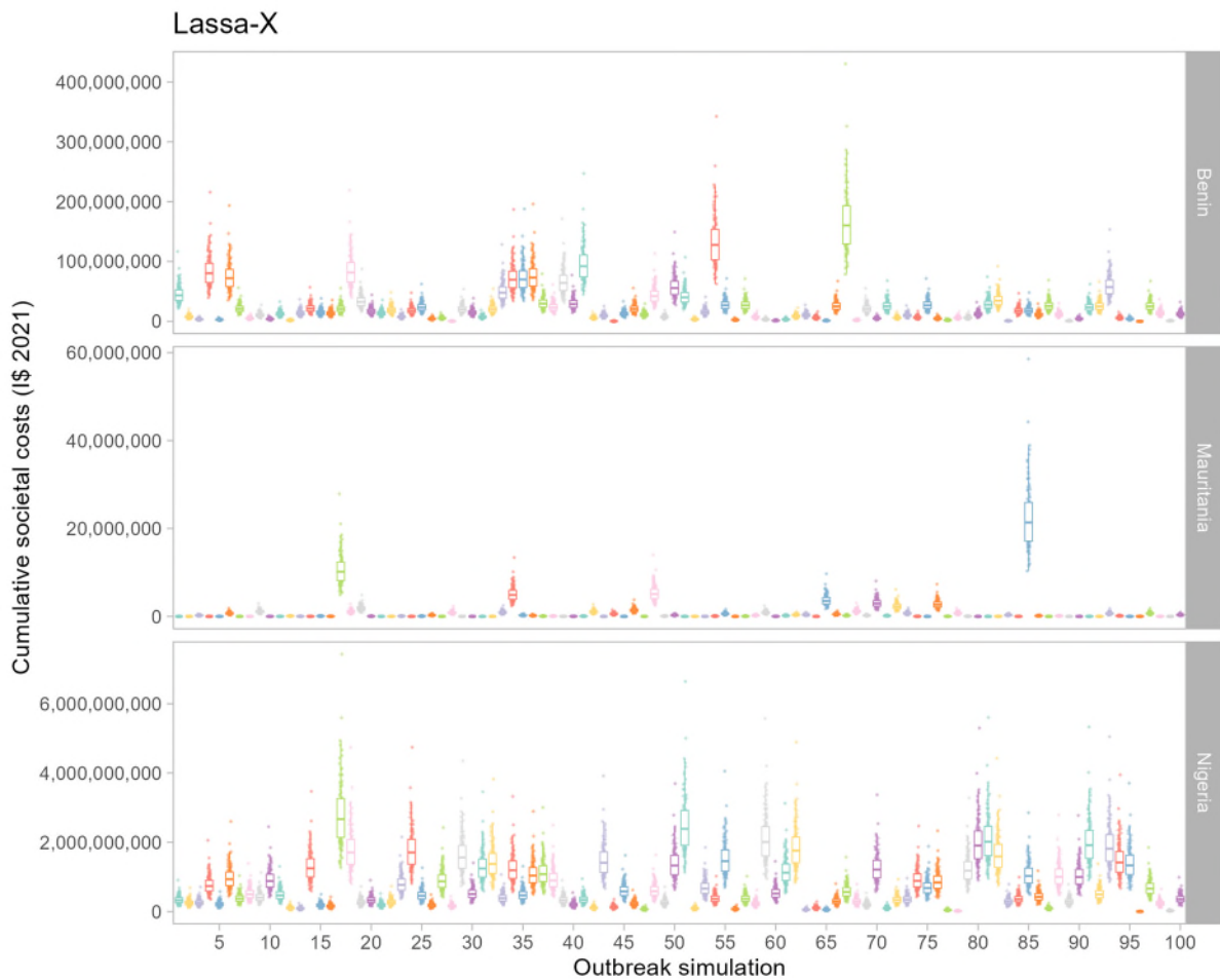
Figure F.2. Raw Lassa-X simulation output data in the absence of vaccination. Raw data points overlaid with boxplots depicting estimates of the cumulative societal costs incurred by Lassa-X across all simulations. The y-axis depicts SC_{\varepsilon, \rho, c} , an estimate of the cumulative societal costs from Lassa-X outbreak simulation \varepsilon (x-axis), Monte Carlo simulation \rho (points) and country c (panels). Results are shown for three selected countries having high estimated burden of Lassa-X (Nigeria), moderate burden (Benin) or low burden (Mauritania). These estimates correspond to baseline parameter assumptions of a 3% annual discounting rate, a probability of sequelae of 62% among patients discharged from hospital, and a ten-fold greater risk of hospitalisation relative to LASV. Upper and lower boxplot whiskers extend no further than values 150% larger or smaller, respectively, than the interquartile range. I\$ = International dollar.
