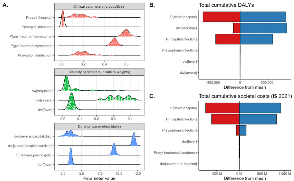
Figure C.2. Input parameter uncertainty and impact on outcomes. (A) Parameter distributions used in Monte Carlo simulations. (B) Tornado plot depicting the mean difference in the total cumulative DALYs due to Lassa fever when using the maximum (blue) or minimum (red) value of corresponding parameters (y-axis). (C) Tornado plot depicting the mean difference in the total cumulative societal costs due to Lassa fever when using the maximum (blue) or minimum (red) value of corresponding parameters (y-axis).
